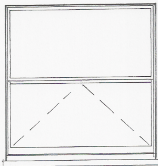
Replacement for window TYPE 8
