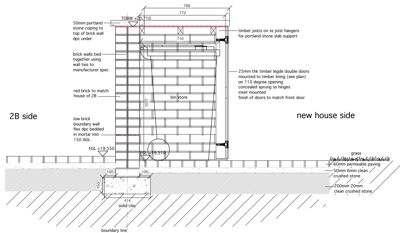
Detail section through brick retaining boundary wall & binstore: section by pavement B-B
