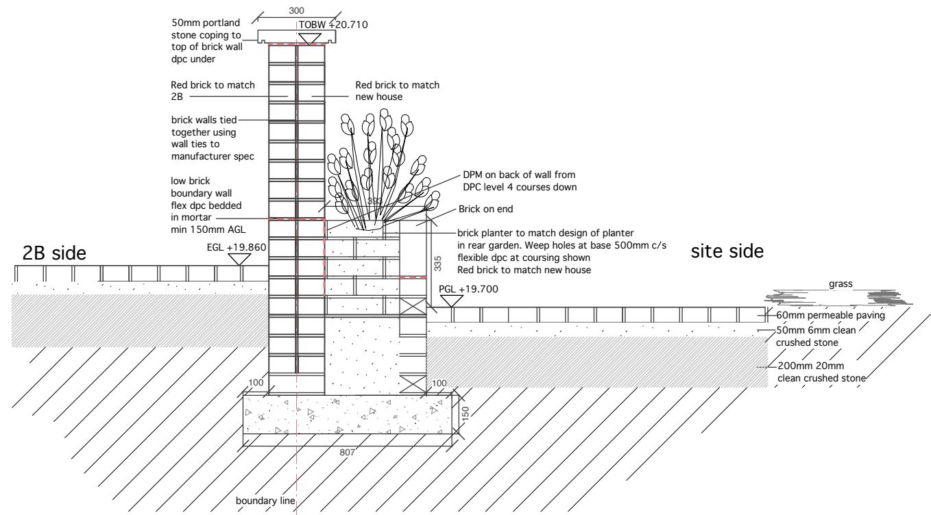
Detail section through brick retaining boundary wall & planter: section by house A-A
