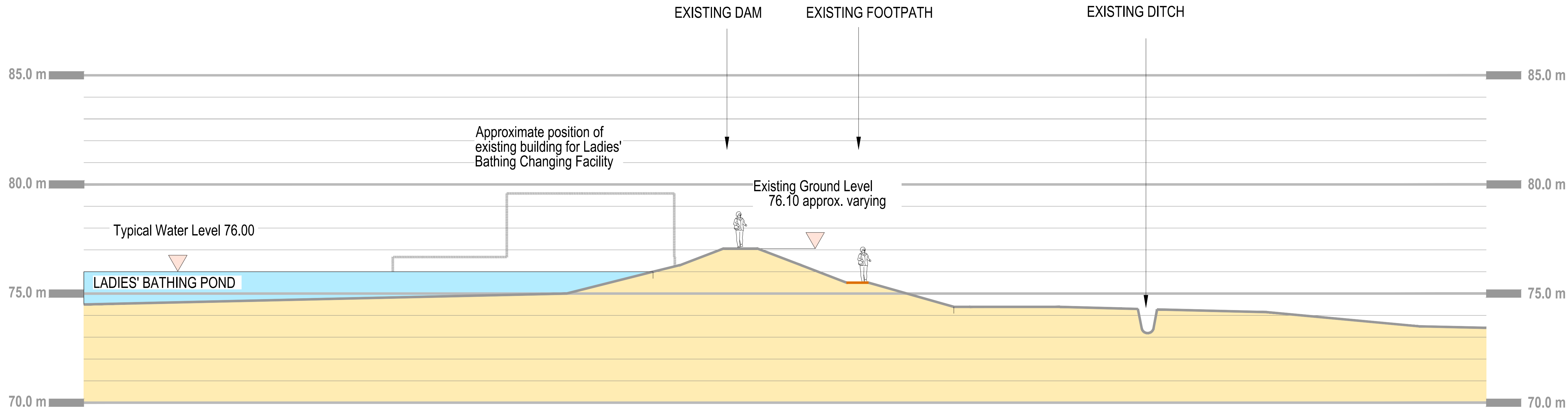
A LADIES' BATHING POND CROSS SECTION SPILLWAY EXISTING P2 7005 SCALE 1: 200@A3
