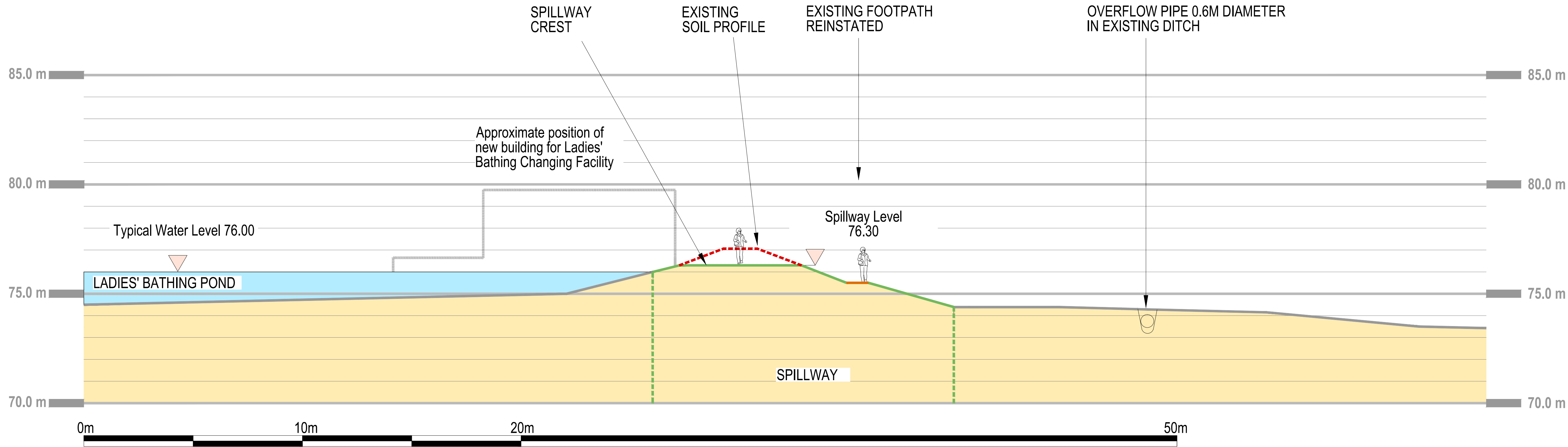
A LADIES' BATHING POND CROSS SECTION SPILLWAY PROPOSED P2 7005 SCALE 1: 200@A3
