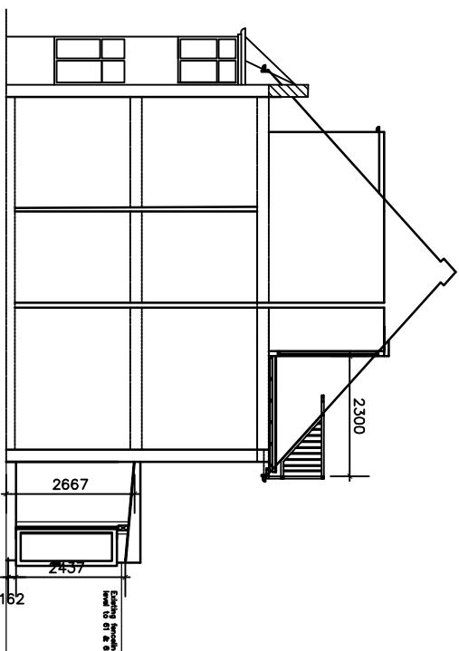
EXISTING SECTIONAL ELEVATION
