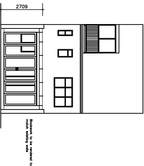
REAR ELEVATION
