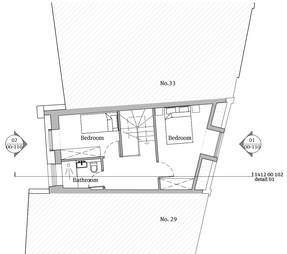
02 Third Floor Plan
