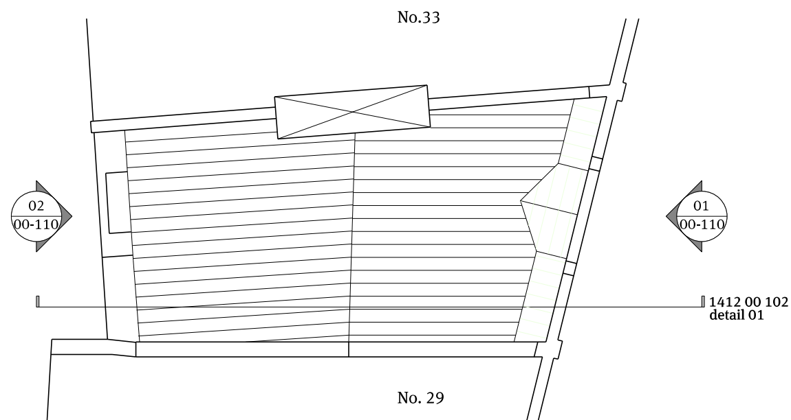
01 Second Floor Plan 1:100@A3
