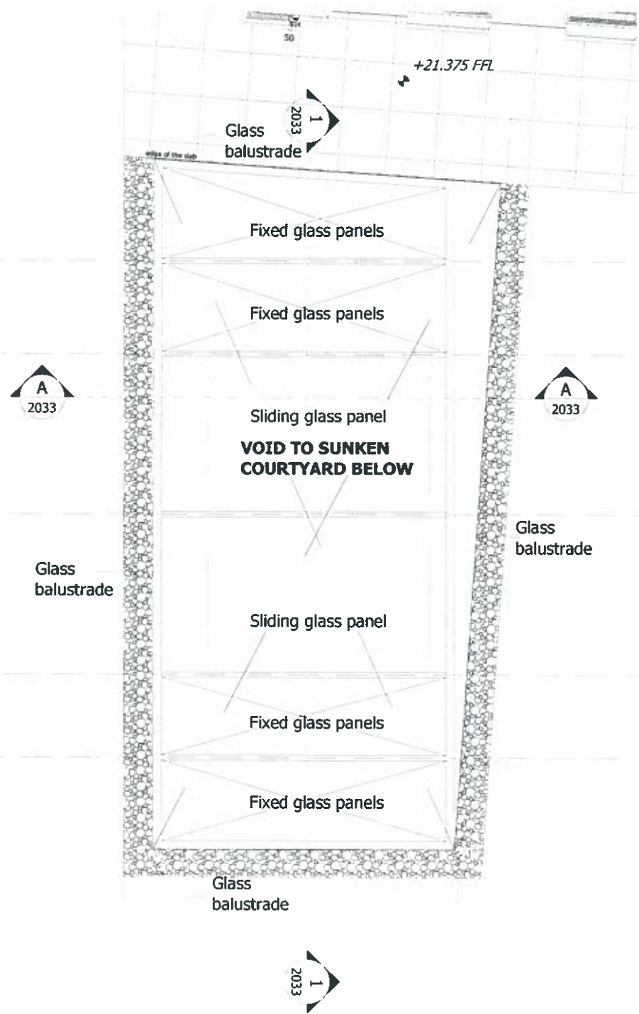
SCALE: 1:50 @ A1 (1:100 @ A0) 1 SUNKEN COURTYARD SETTING OUT PLAN
