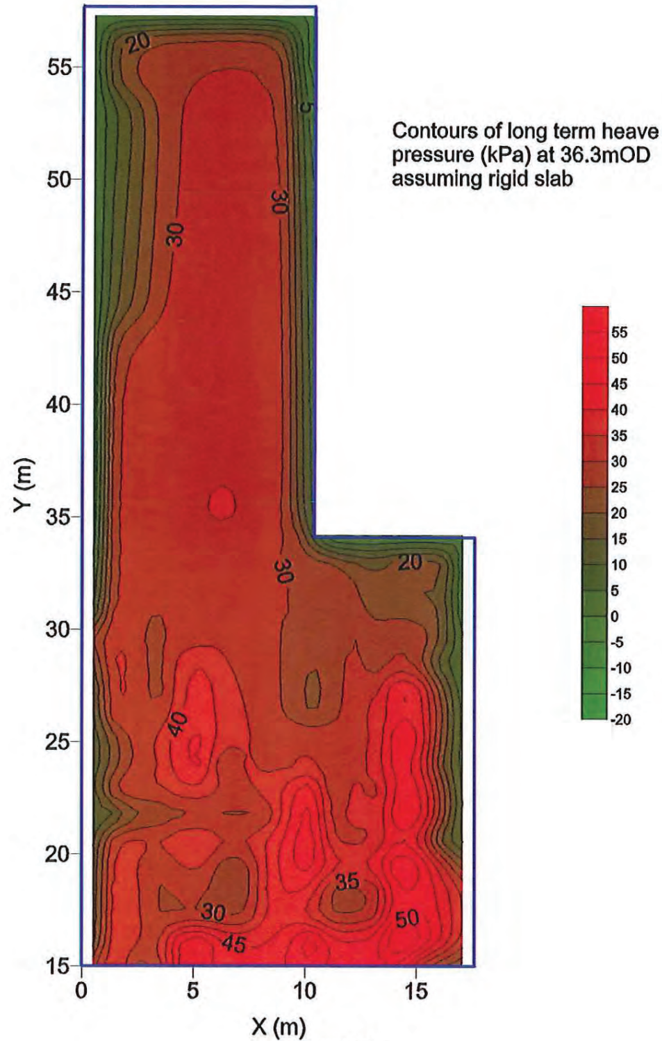
Figure 14 (Predicted heave pressure (kPa) for a fully rigid basement slab)
