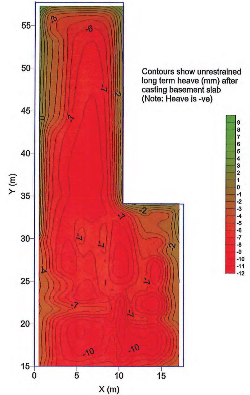
Figure 13 (Predicted heave (mm) for a fully flexible basement slab)
