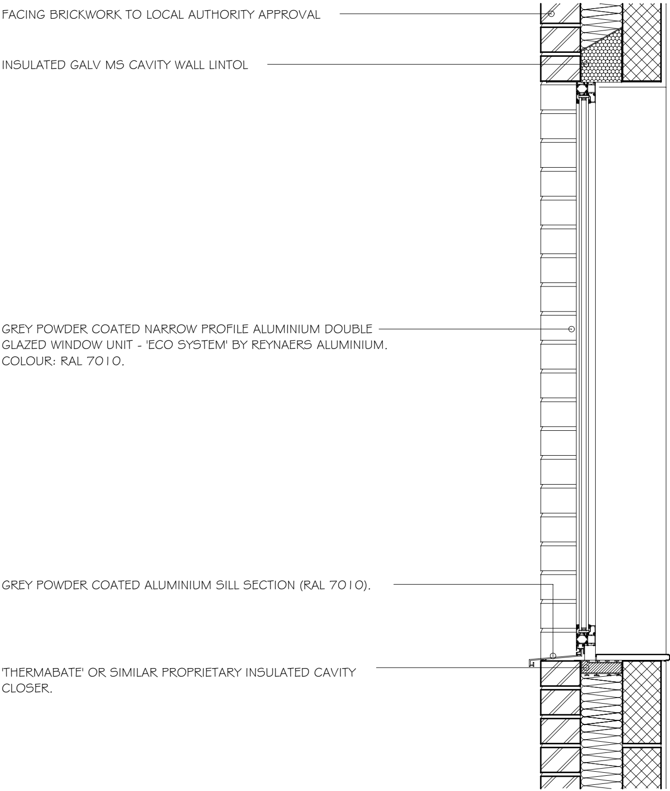
typical window section
