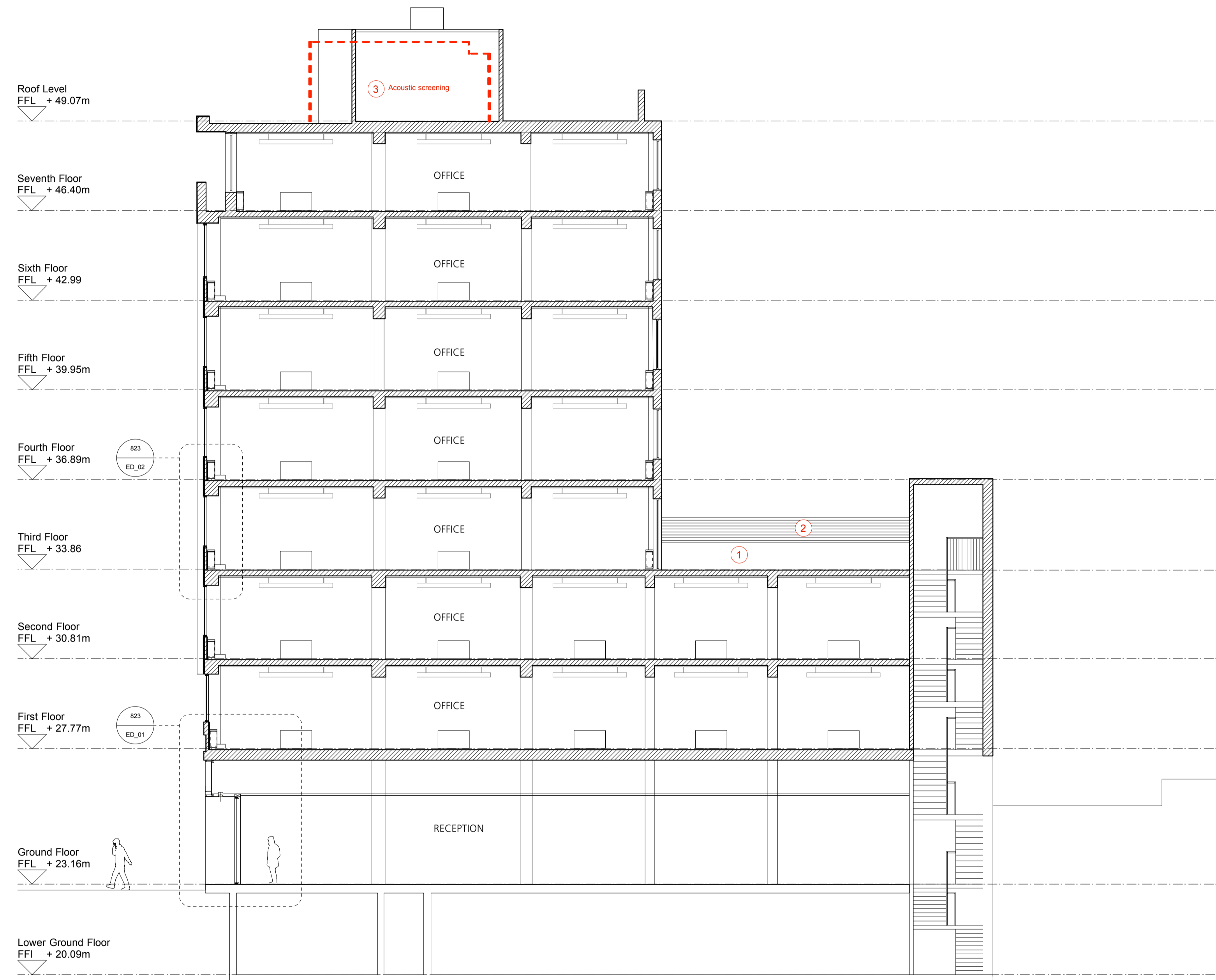
01 Proposed Section AA GS_AA 1:100
