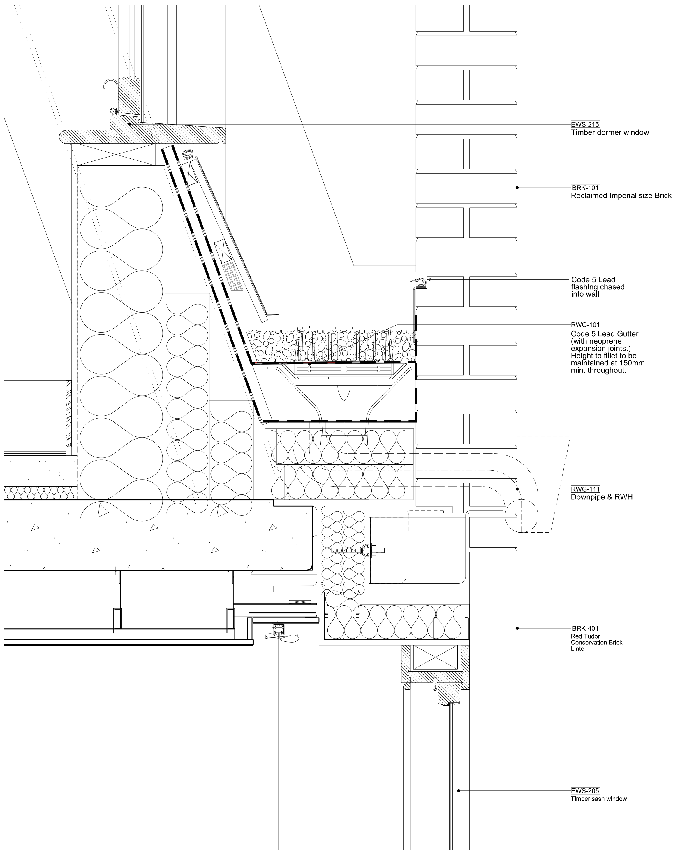
01 Section: East Mansard Roof 1:5
