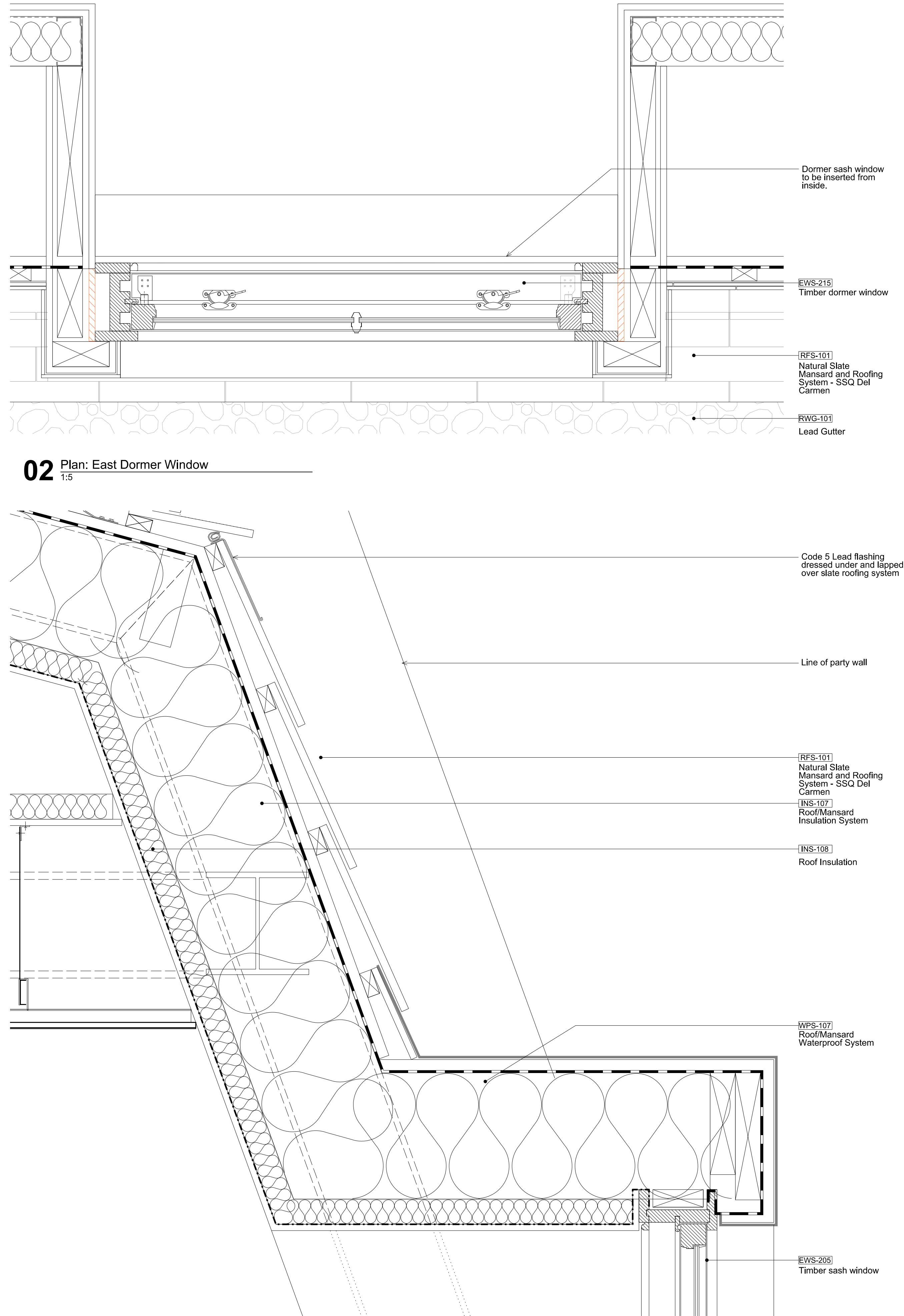
03 Section : East Mansard Roof 1:5
