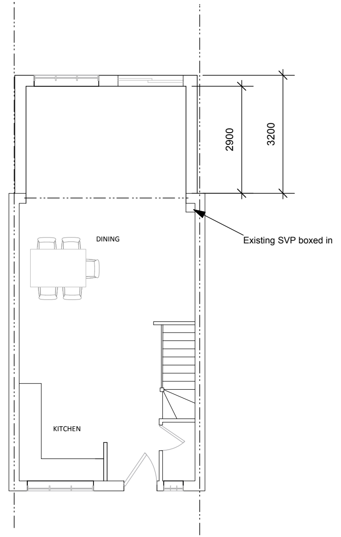
Proposed Ground Scale: 1:100
