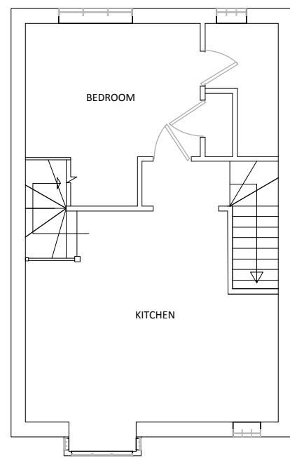
Existing Second Scale: 1:100
