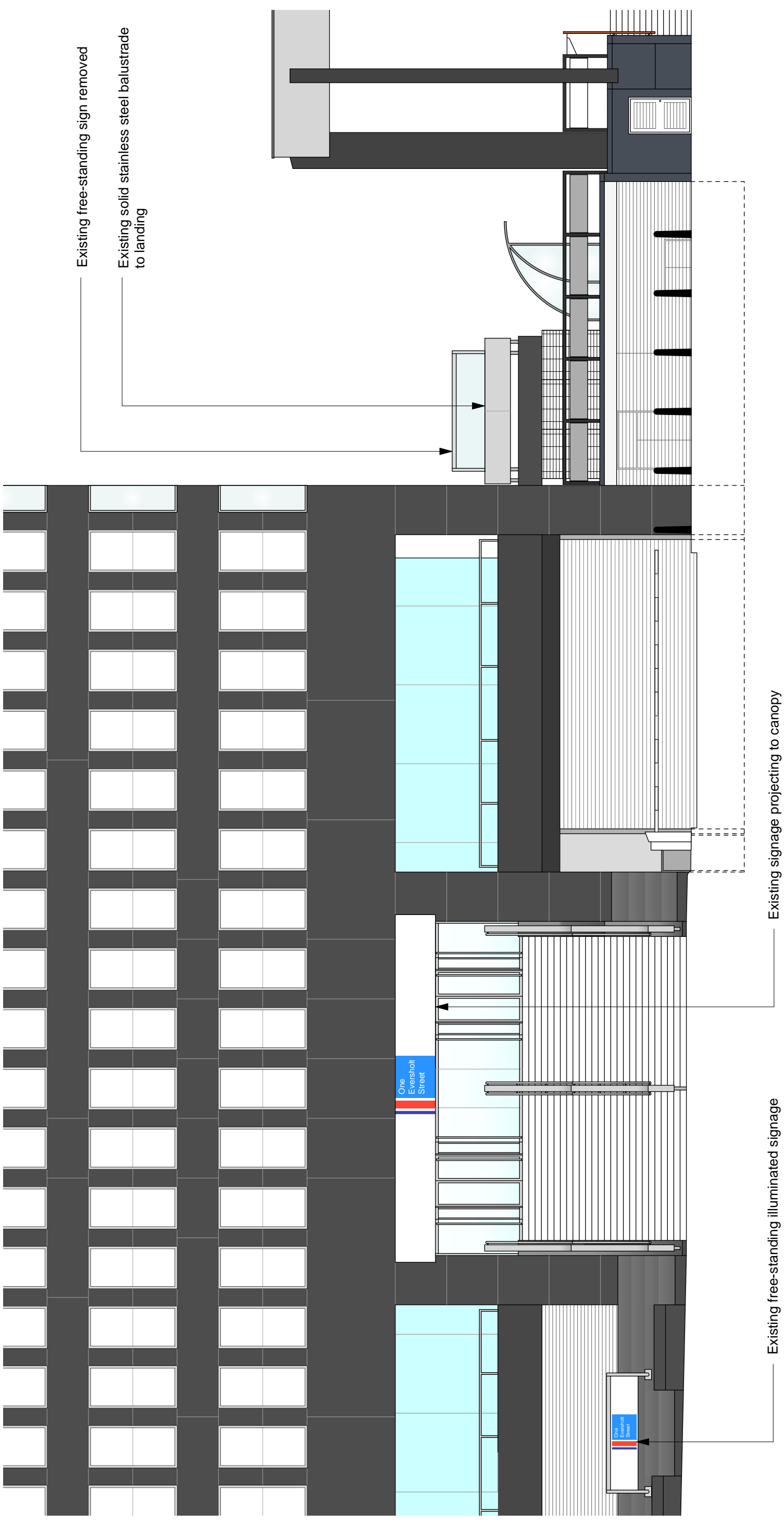
01 One Eversholt Street - Existing East Elevation Scale 1:100@A3
