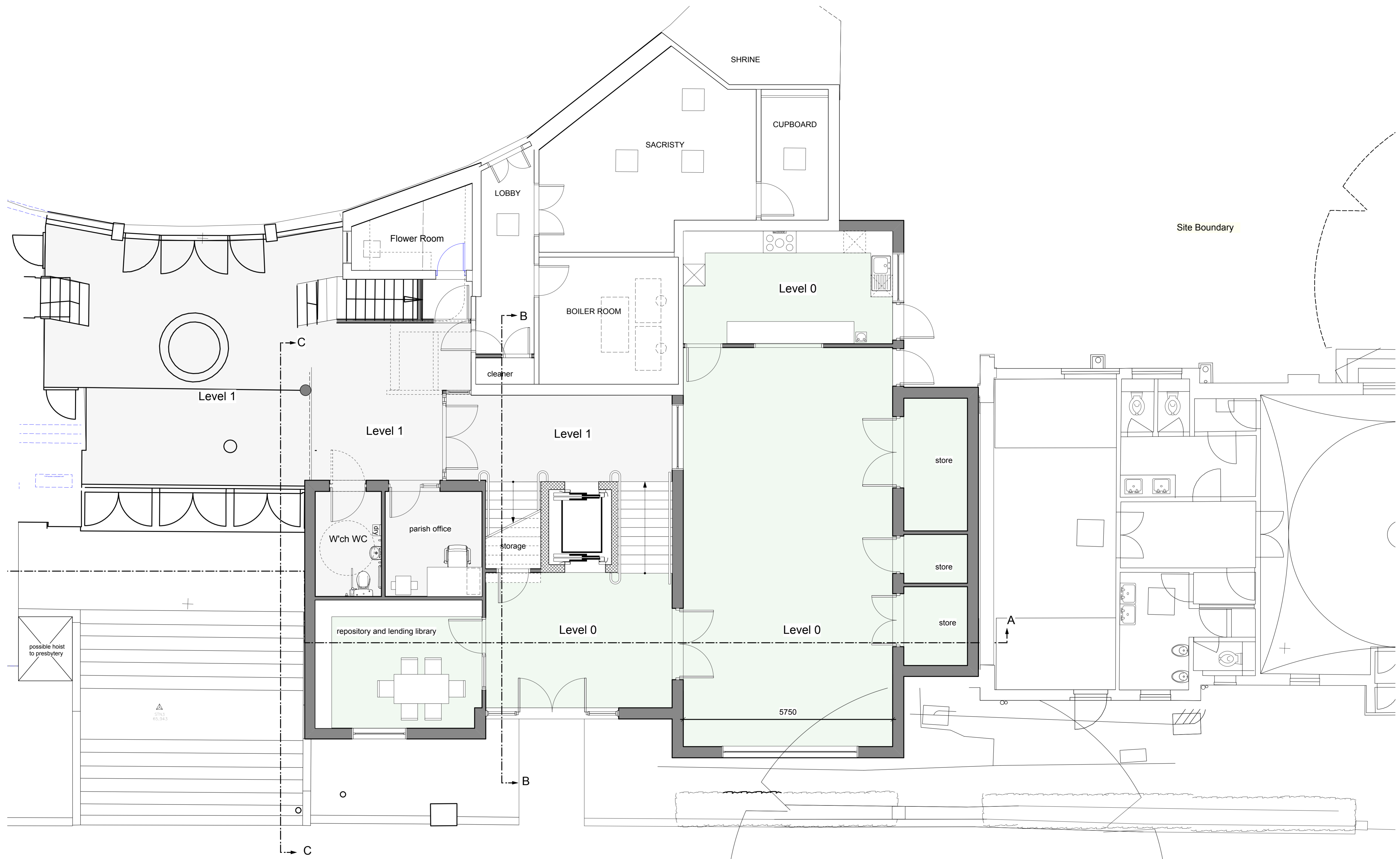
Proposed Ground Floor
