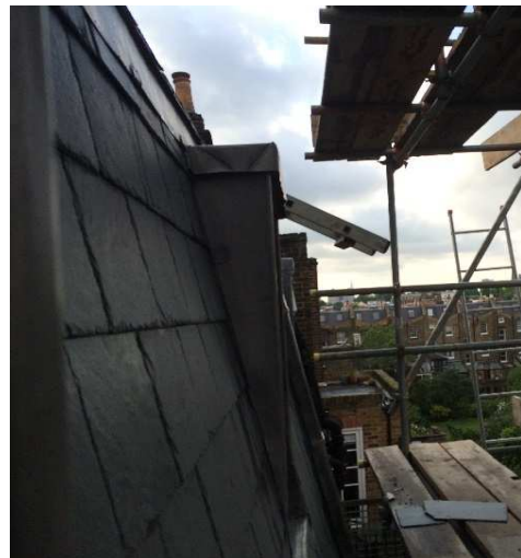
Photo 02 & 03 Proposed roof, natural slates with Lead Dormers
