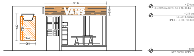
1 FACADE E-E
