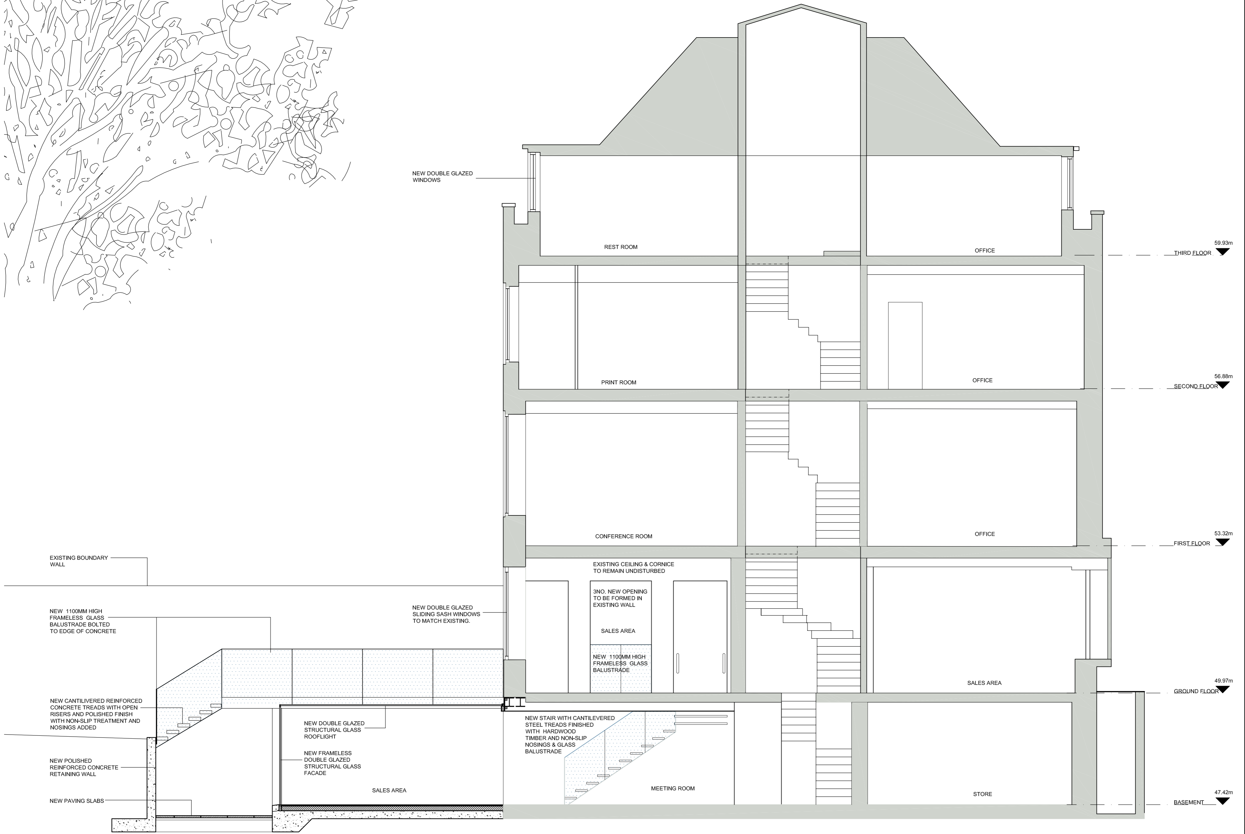
SECTION B-B
