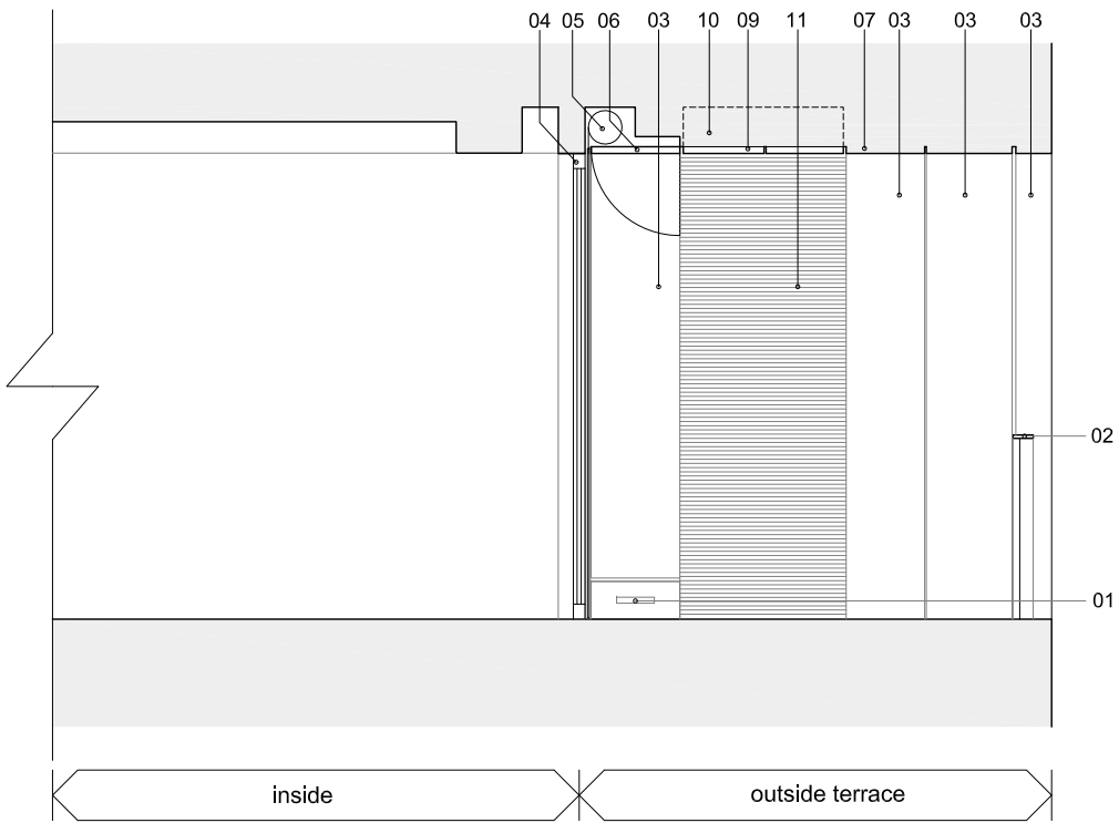
section 2 - security shutter closed
