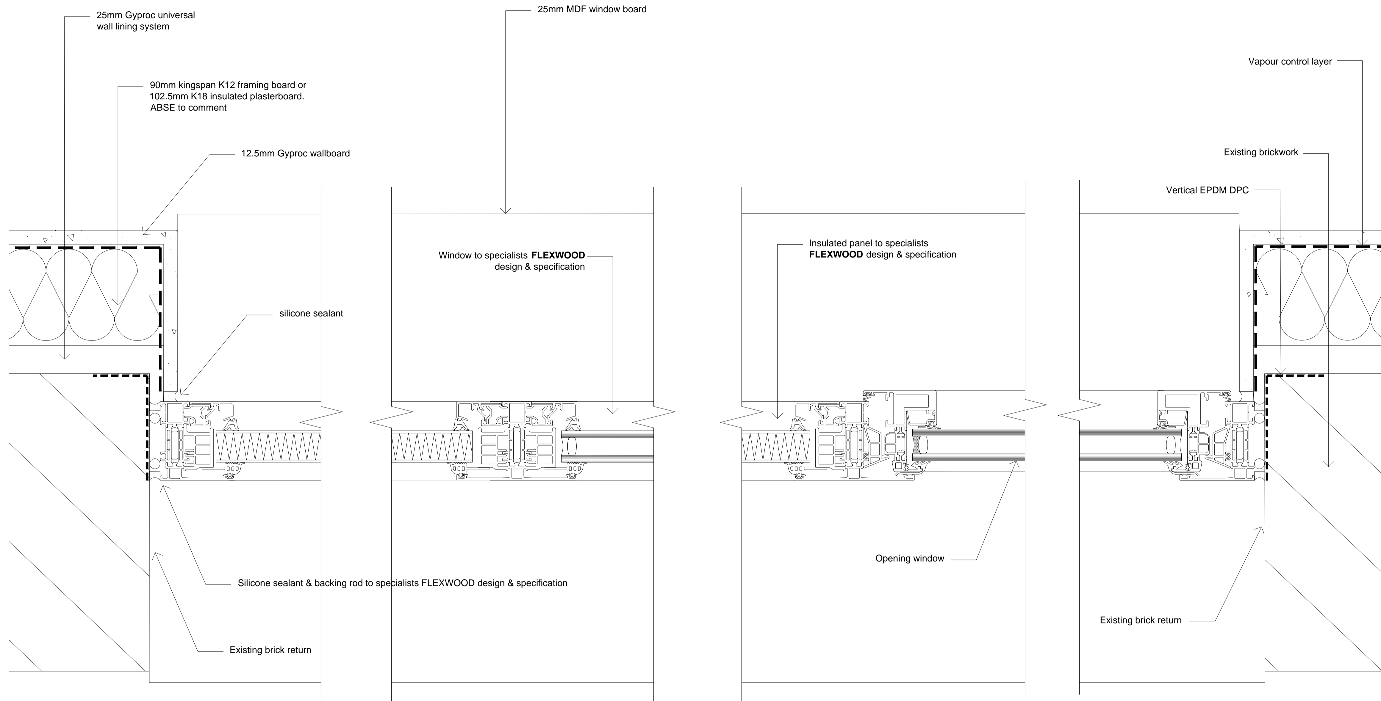
1 Insulated Panel Jamb Detail
