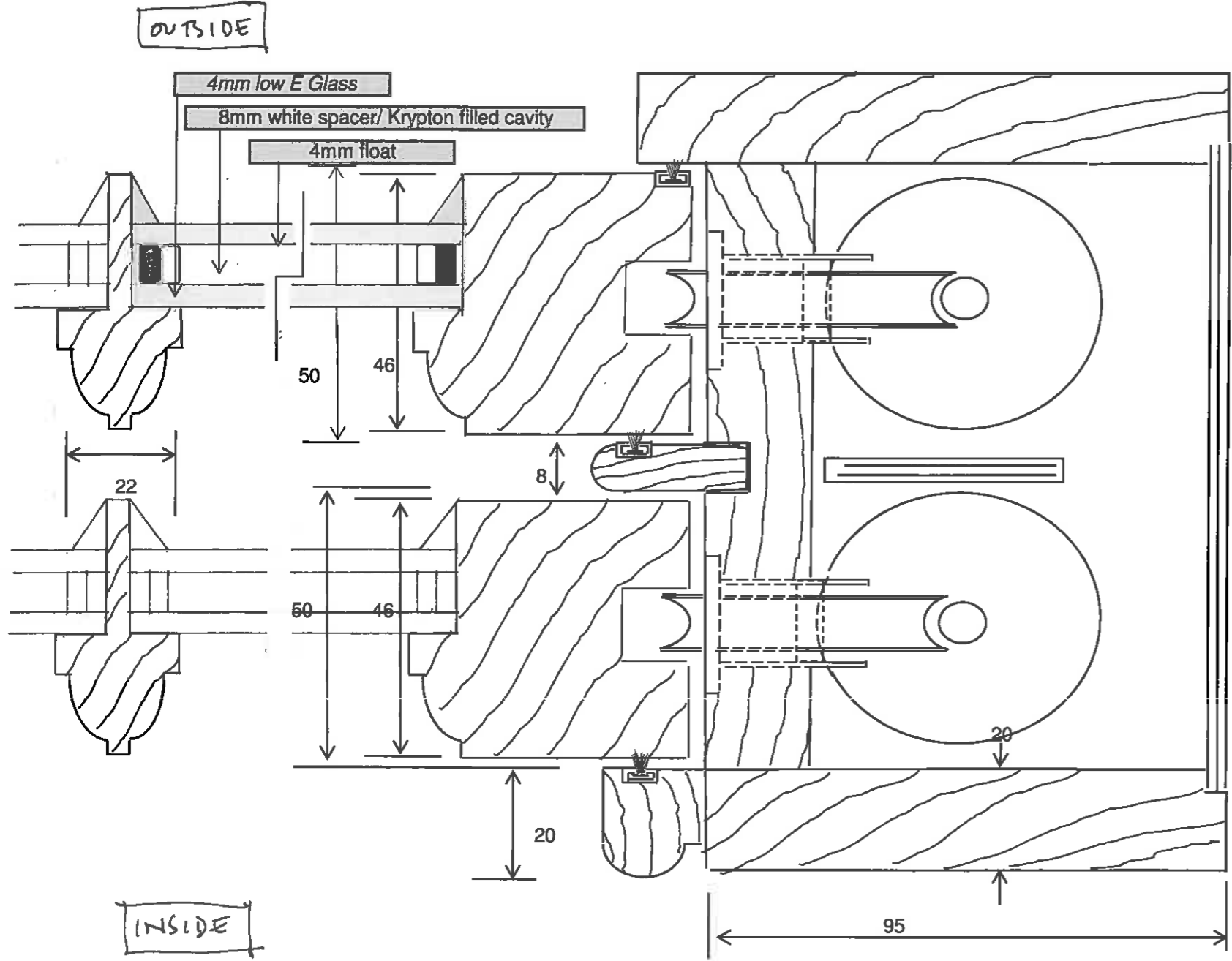
Section of Sash Stile Glazing Bar and Sash box
