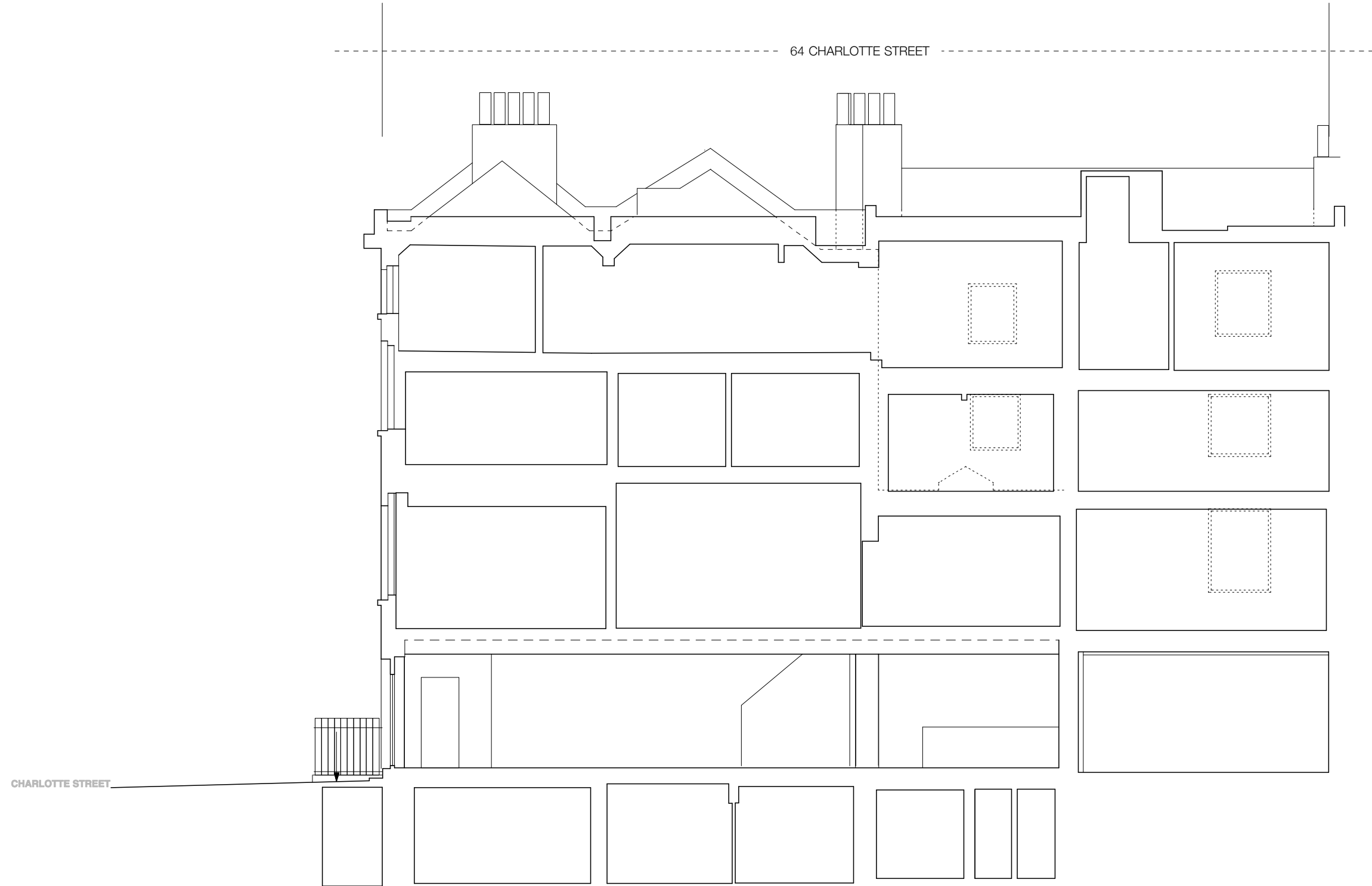
EXISTING SECTION AA
