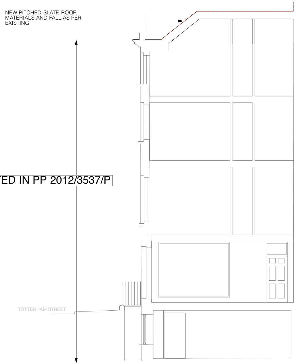
PROPOSED SECTION BB
