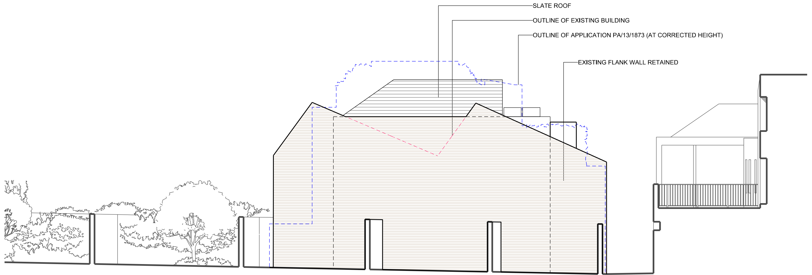
PROPOSED SIDE ELEVATION FROM GARDENS IN LADY SOMERSET ROAD - 1:100 @ A3
