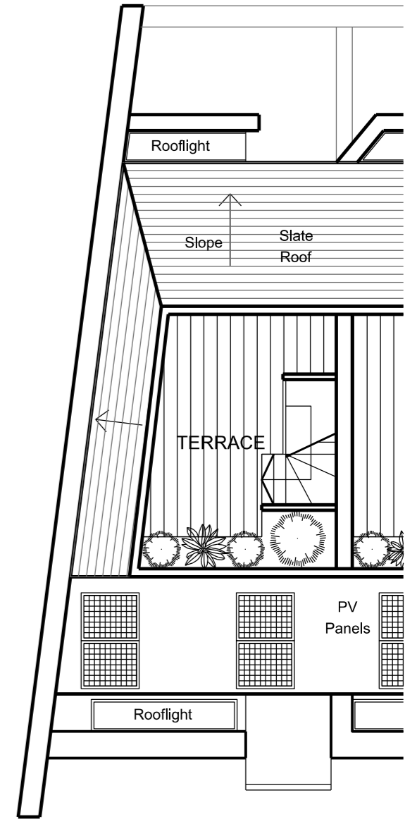
ROOF PLAN
