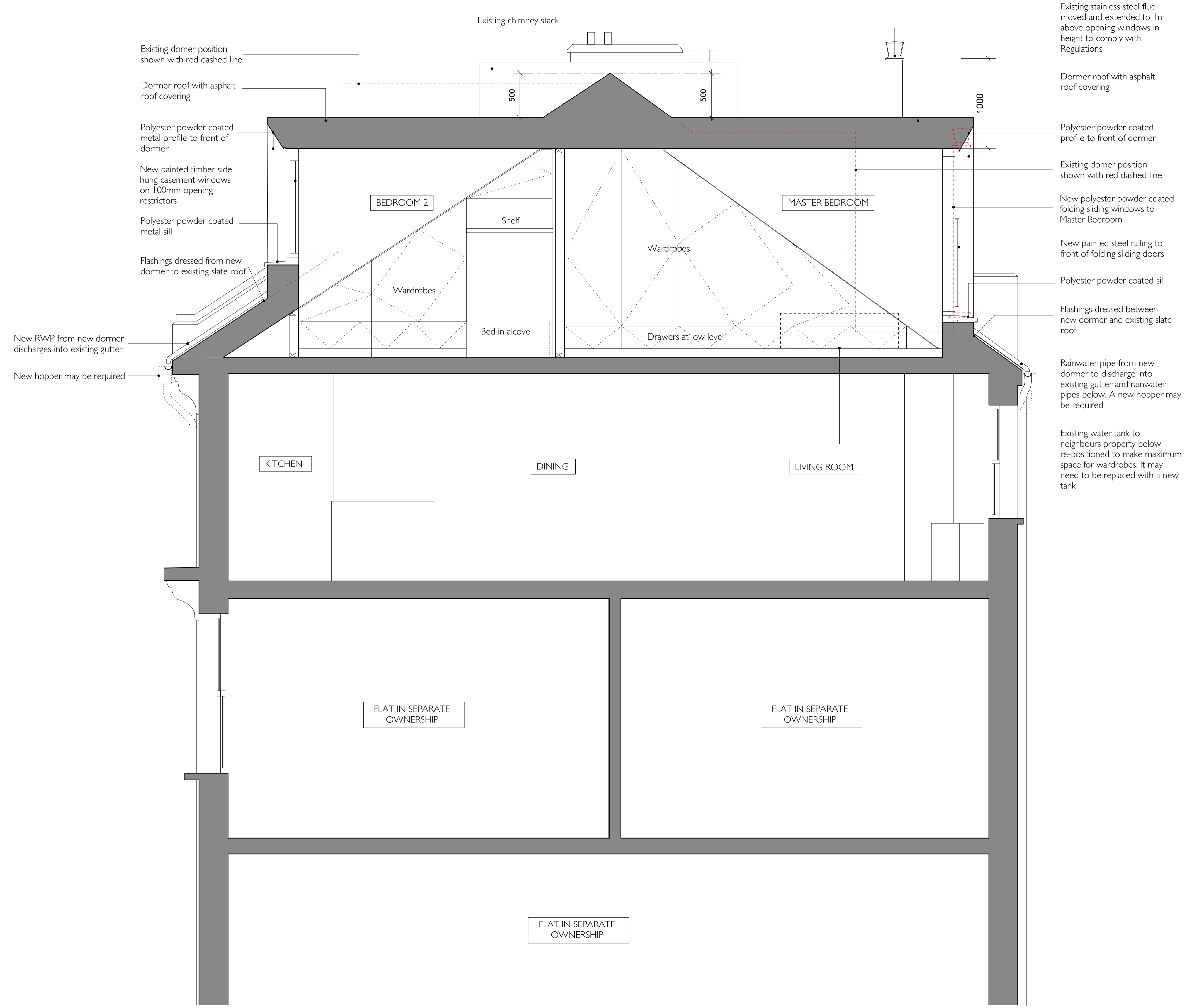
GA-012 - PROPOSED SECTION C-C 1:25
