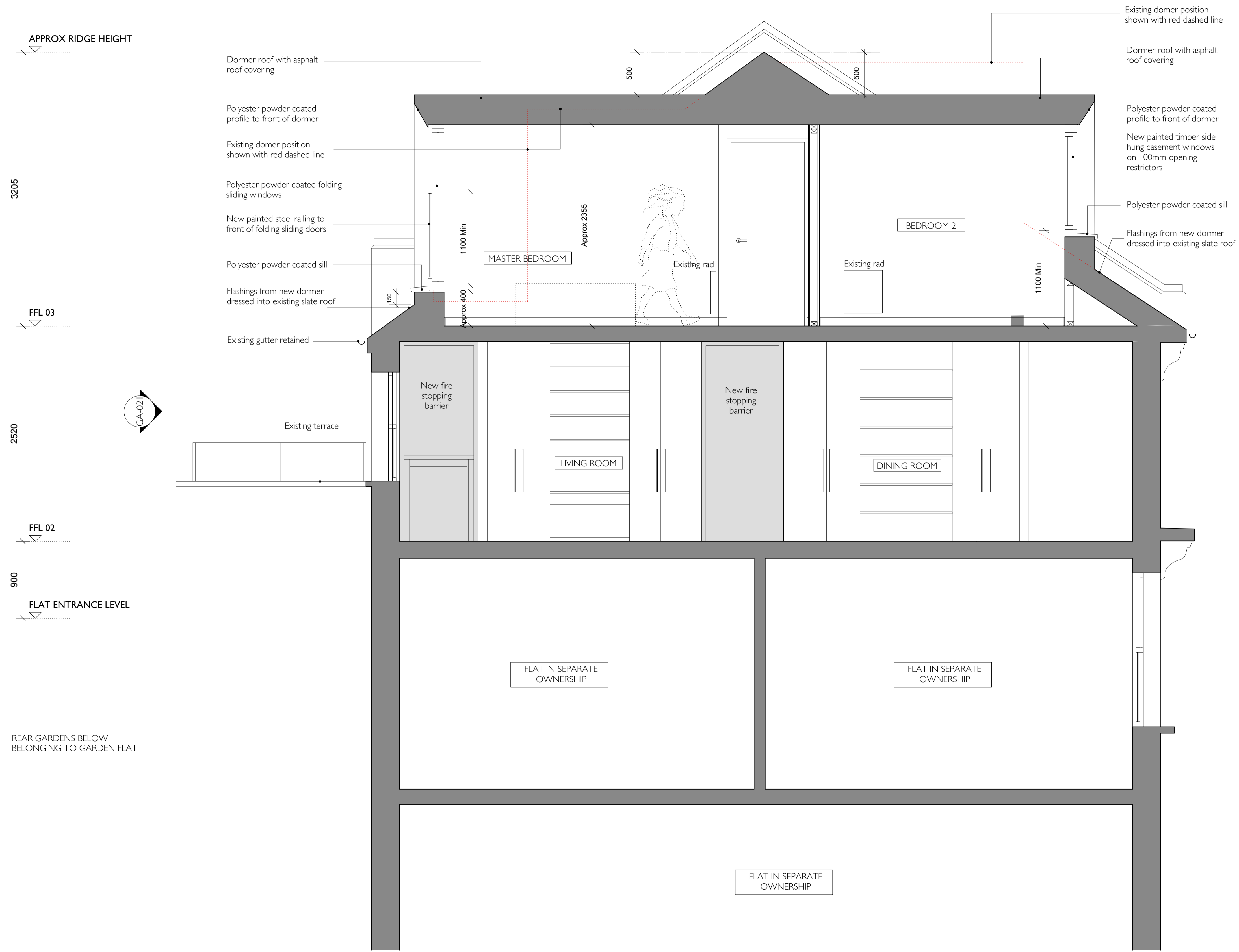
PROPOSED SECTION B-B 1:25 GA-011
