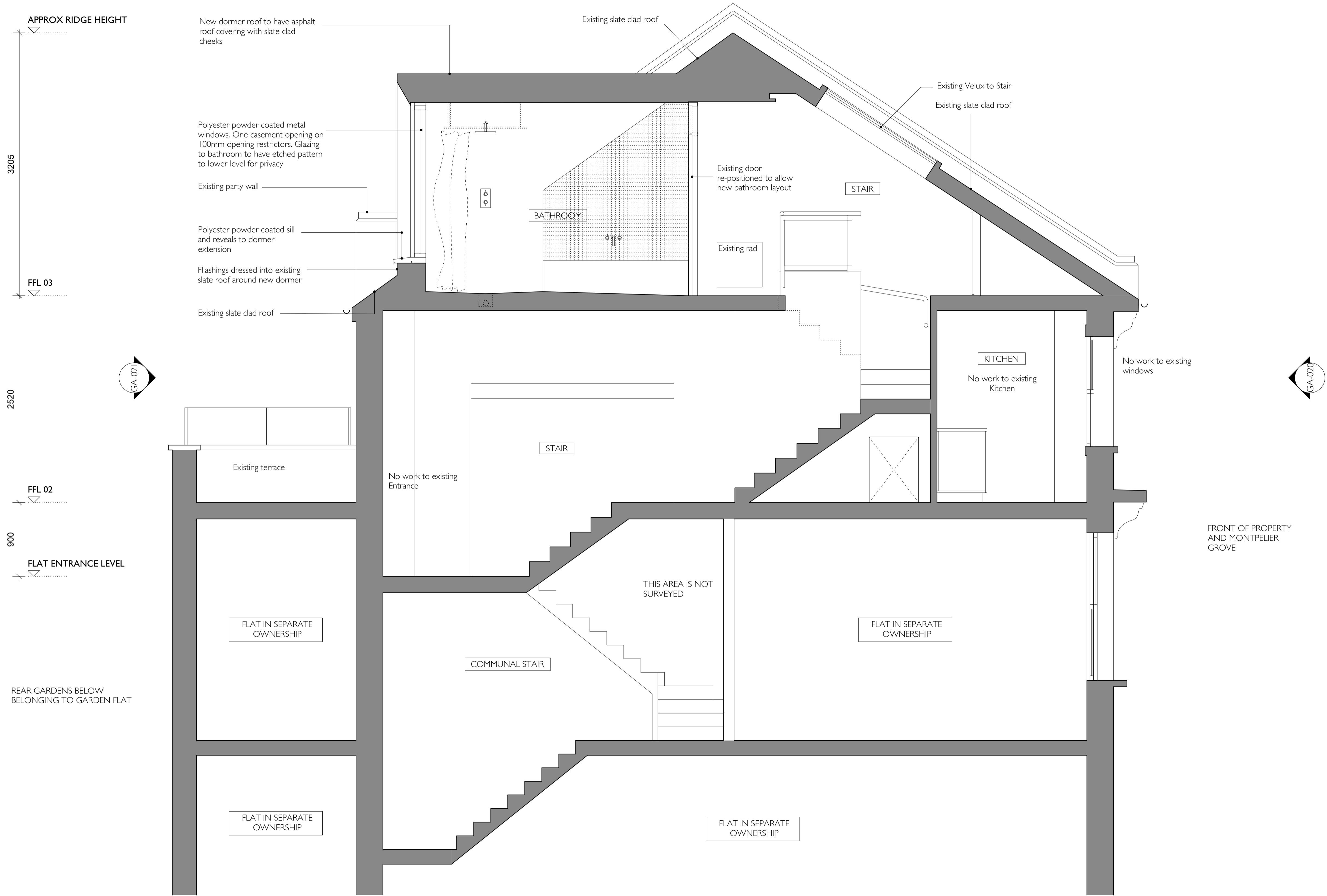
PROPOSED SECTION A-A 1:25 GA-010
