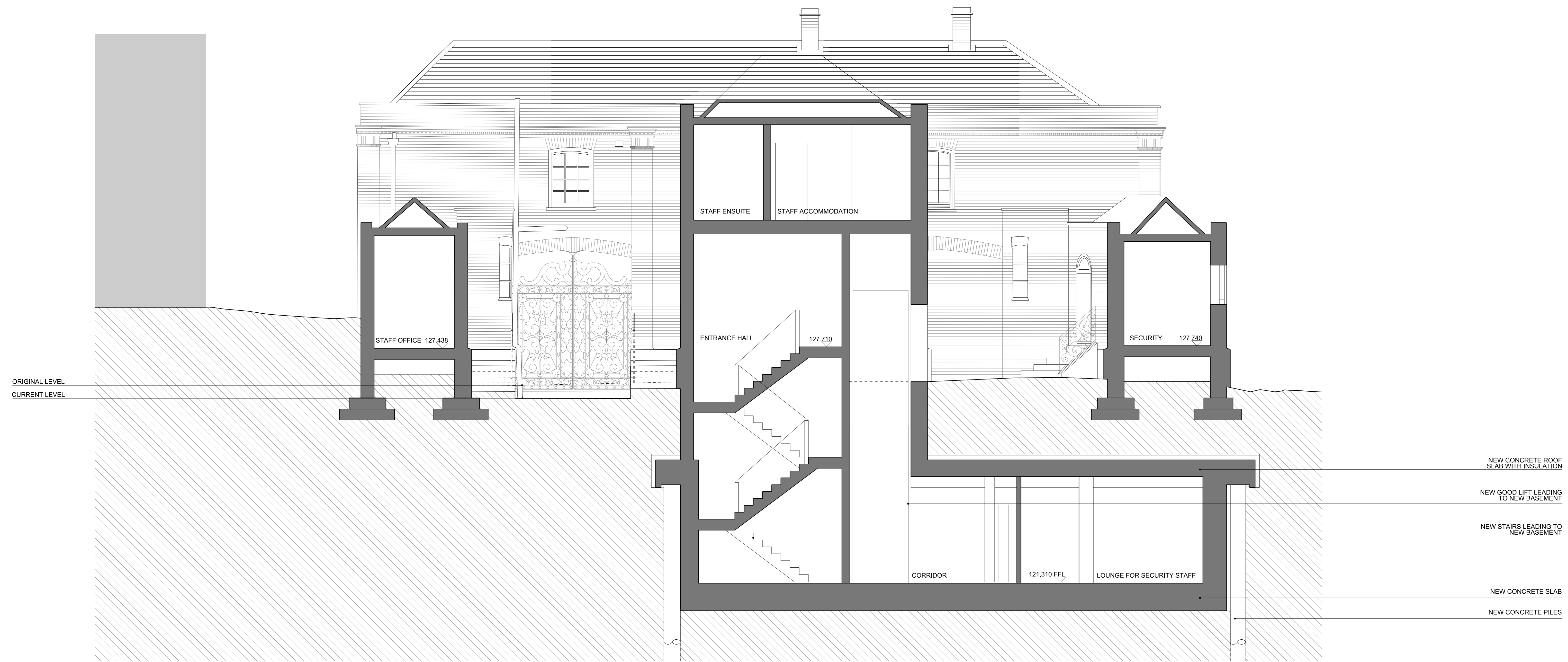
01 SECTION QQ 1:50 @ A0
