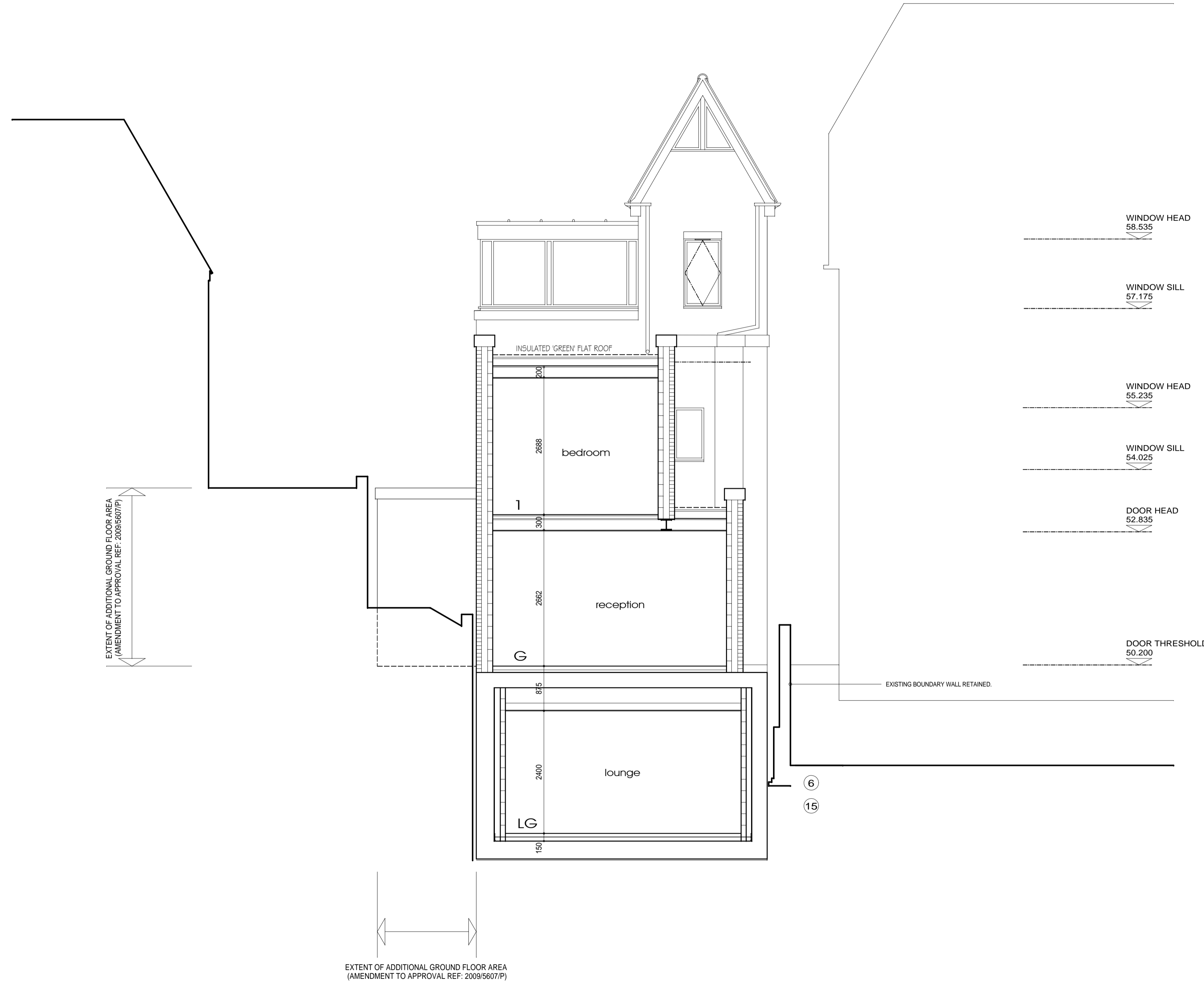
section aa
