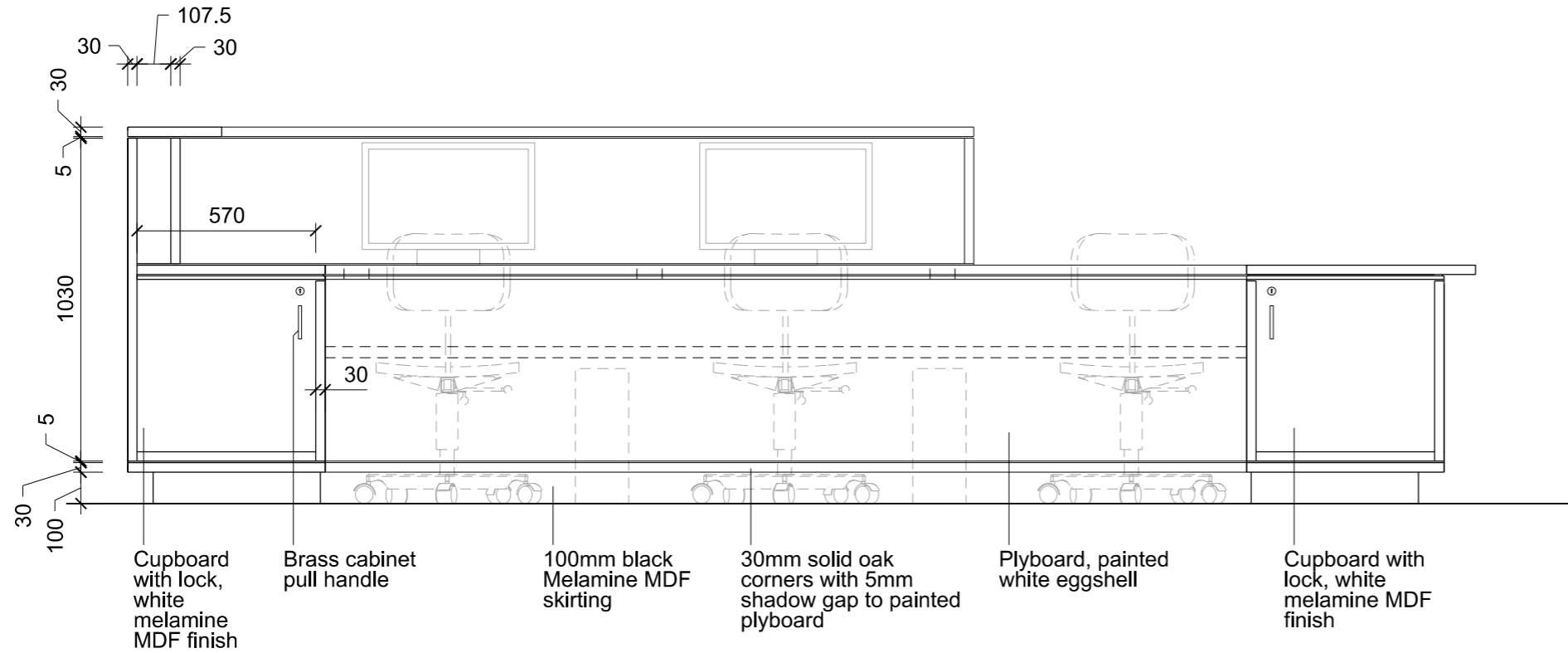
01 Elevation C Reception Desk Details
