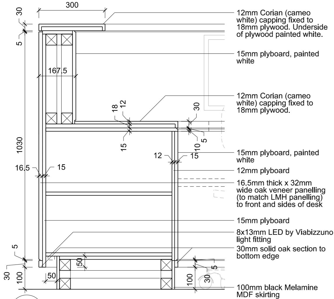
02 Section through cupboard Reception Desk Details
