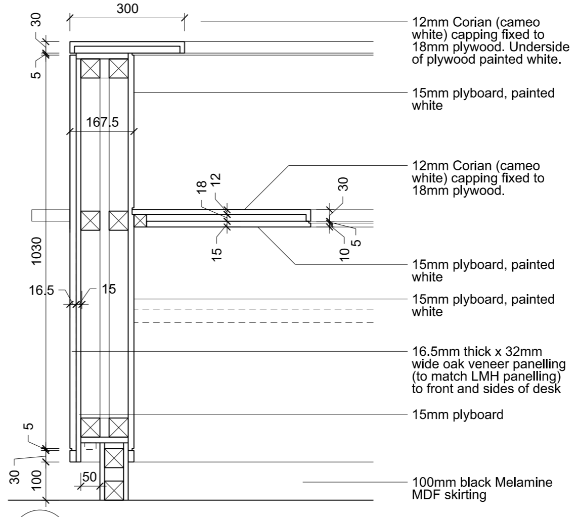
03 Section through counter Reception Desk Details
