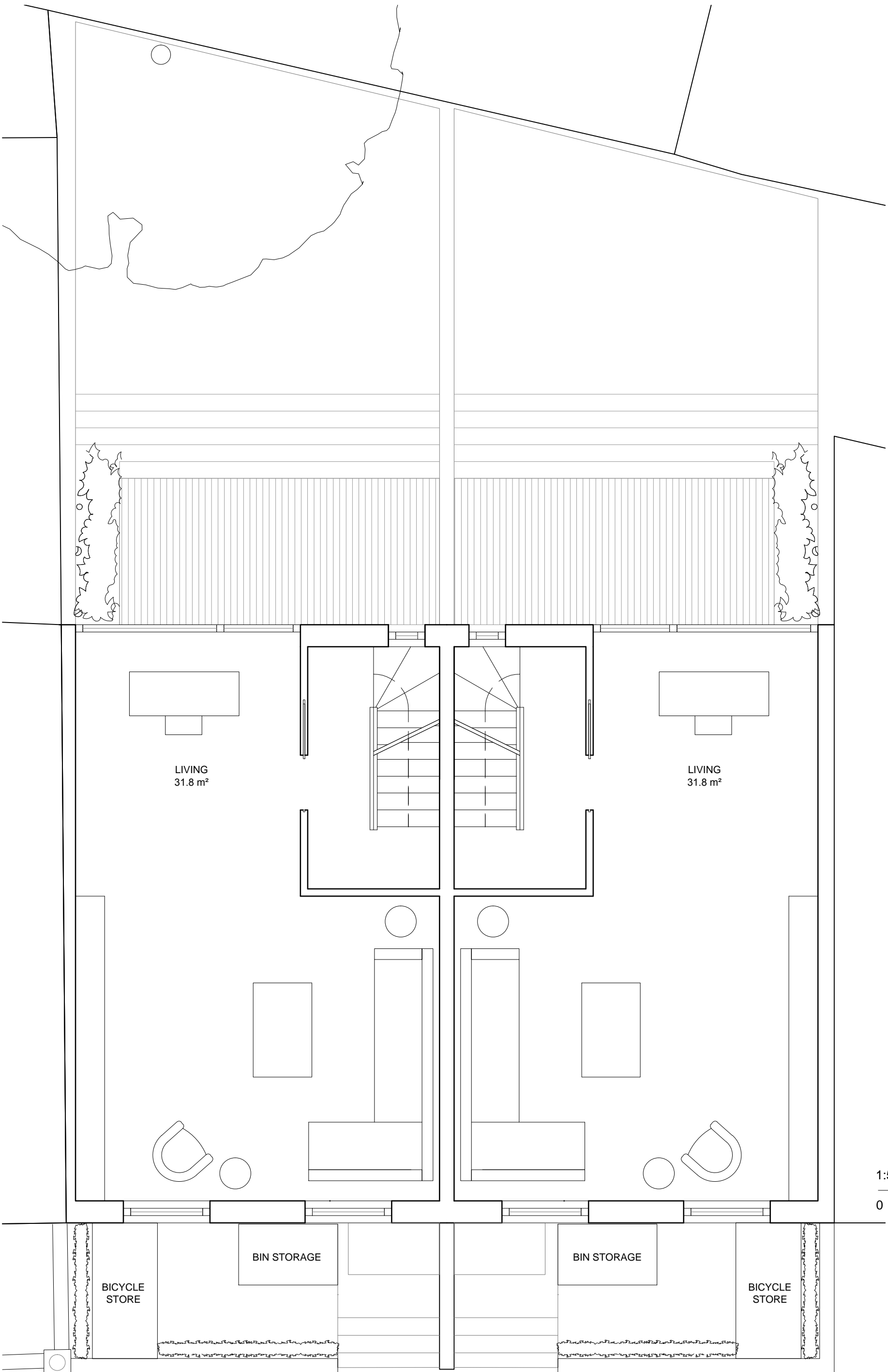
FIRST FLOOR GIA_ 38.3 m 2
