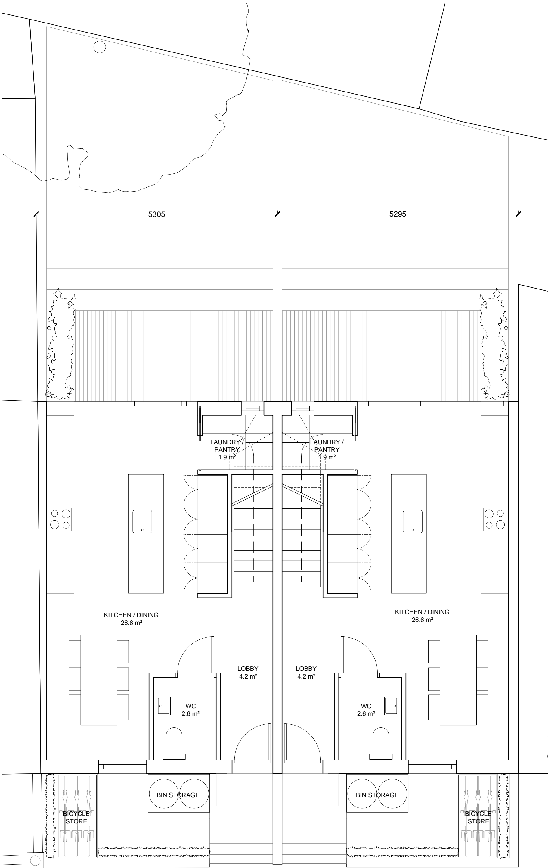
GROUND FLOOR GIA 37.7 m 2
