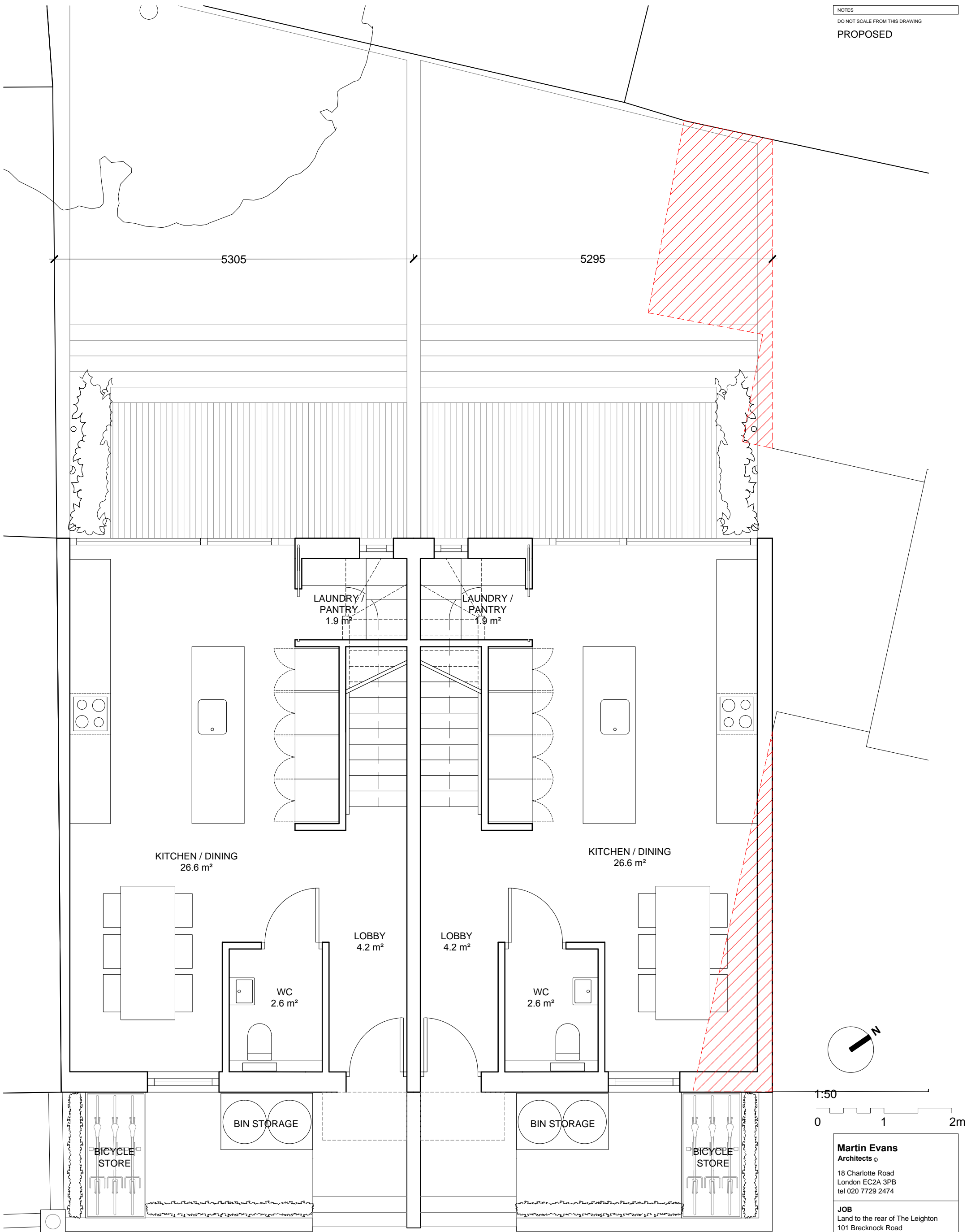
GROUND FLOOR GIA_ 37.7 m 2
