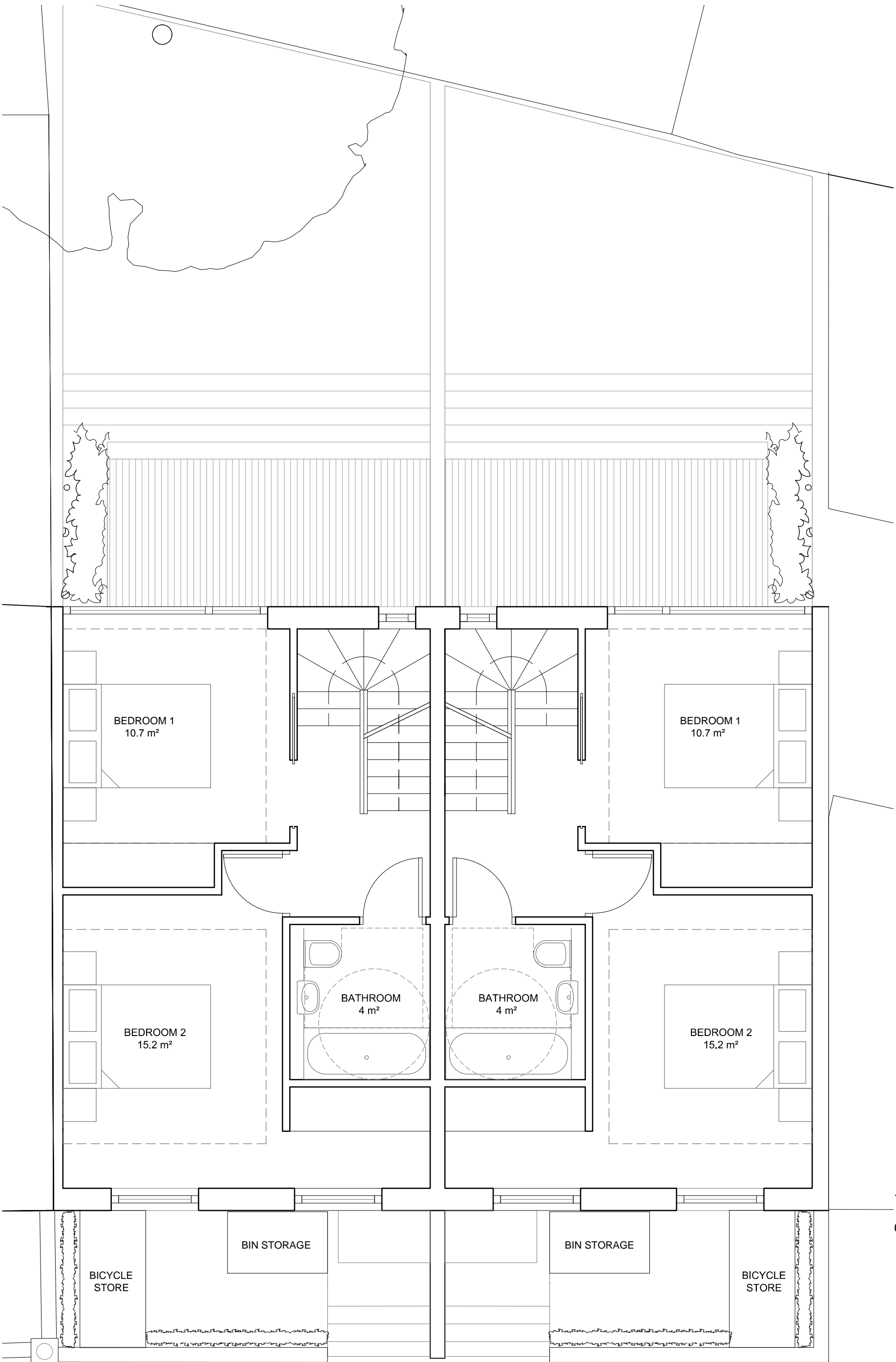
SECOND FLOOR GIA_ 37.64 m 2
