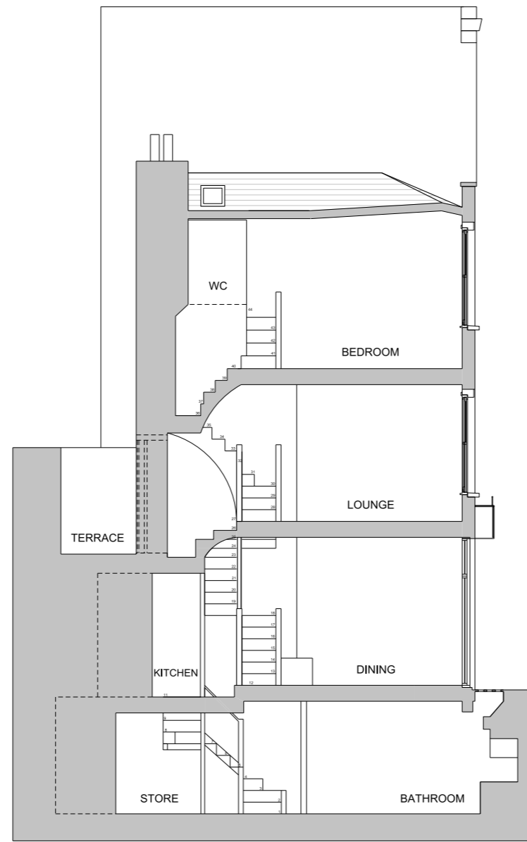
SECTION AA
