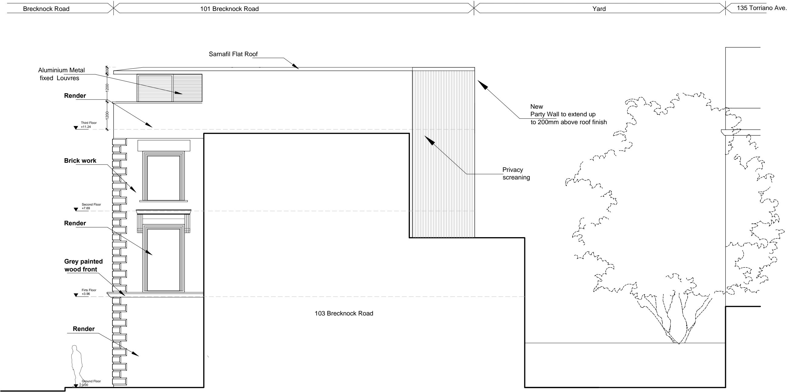
SIDE ELEVATION 1/100
