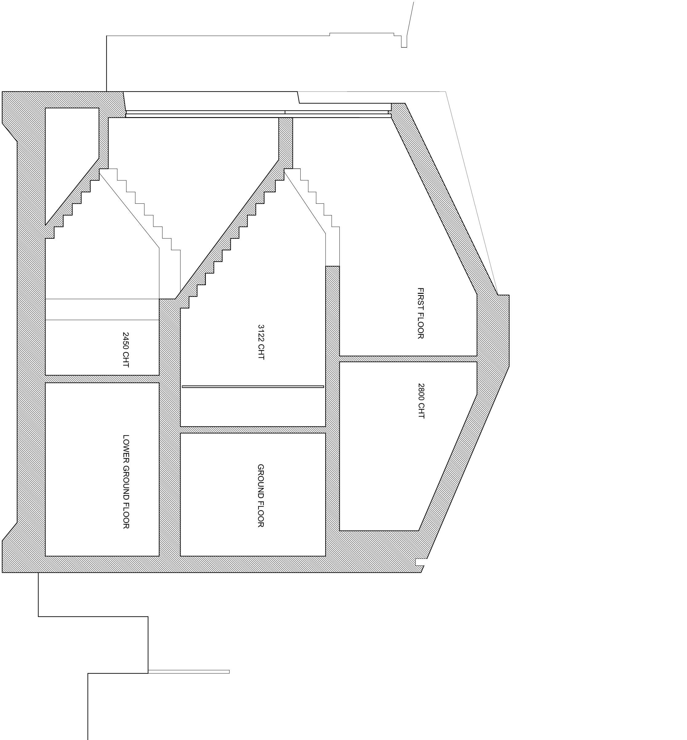
PROPOSED SECTION A-A
