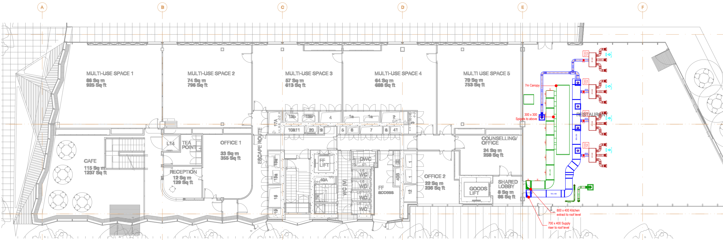
DIORAMA - GROUND FLOOR PART PLAN
