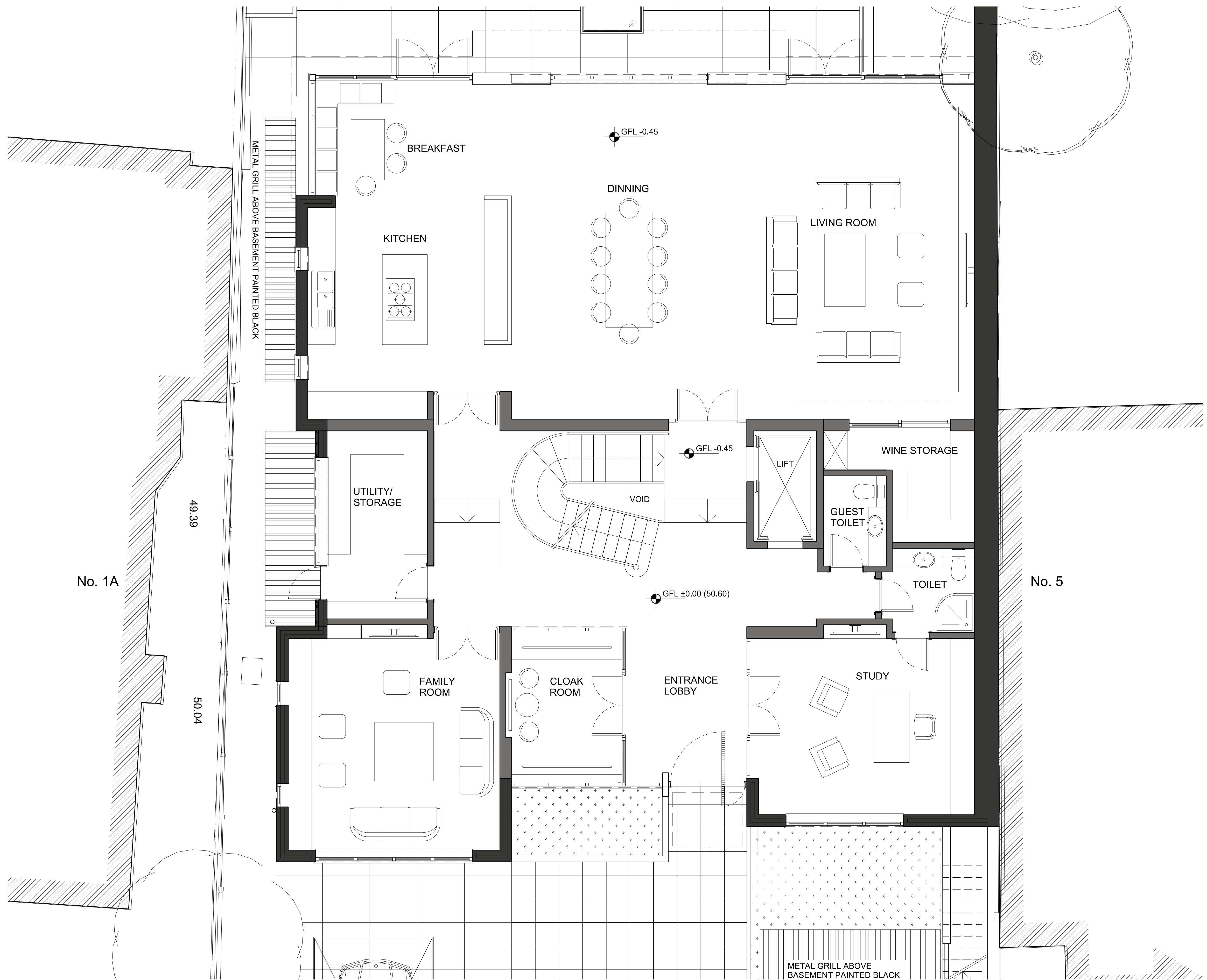
PROPOSED GROUND FLOOR Scale 1:50
