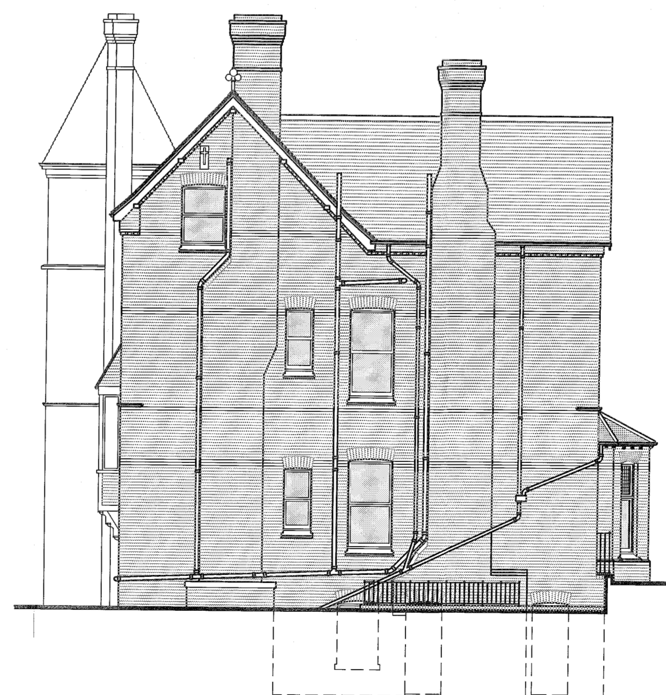
North Elevation
