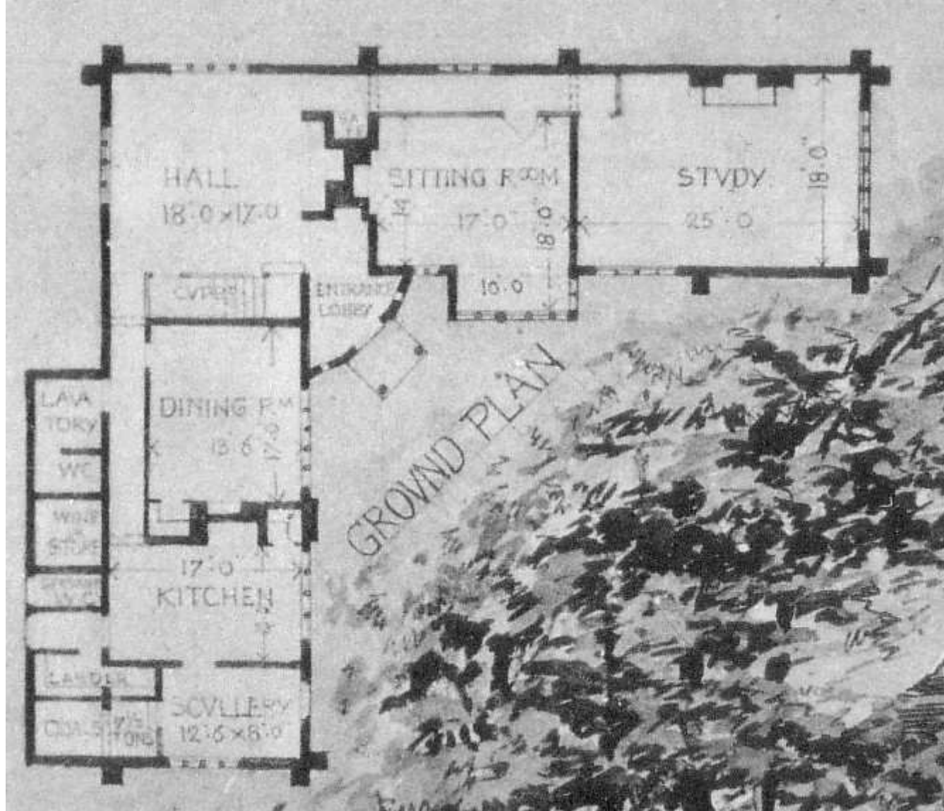
Ground Plan, RIBA Drawings Collection, fig. 6
