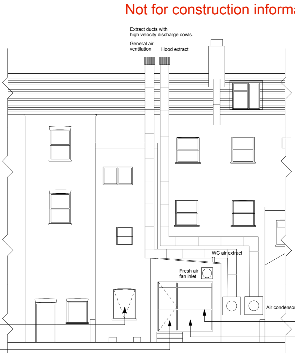
Rear Elevation- Proposed
