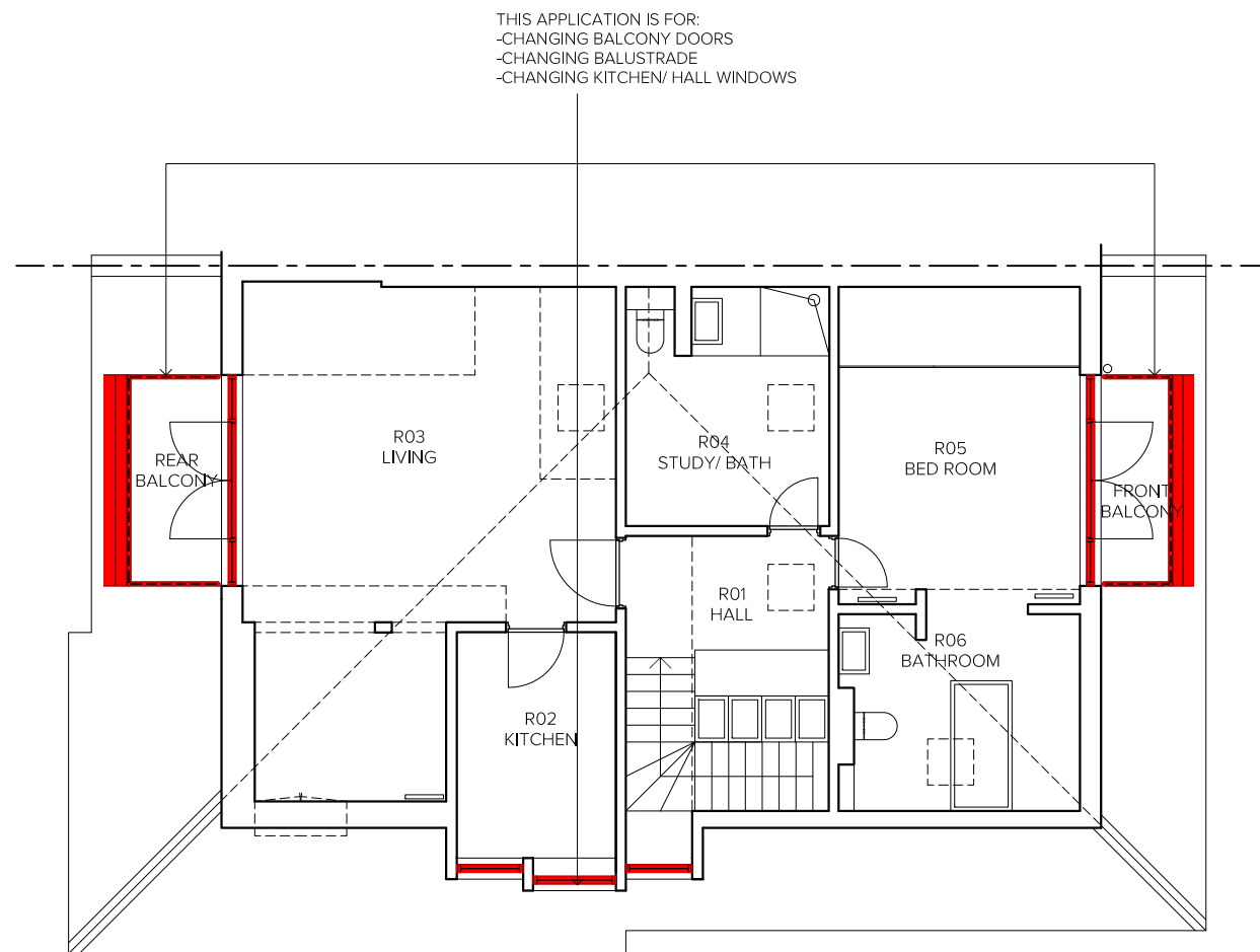
EXISTING THIRD FLOOR PLAN
