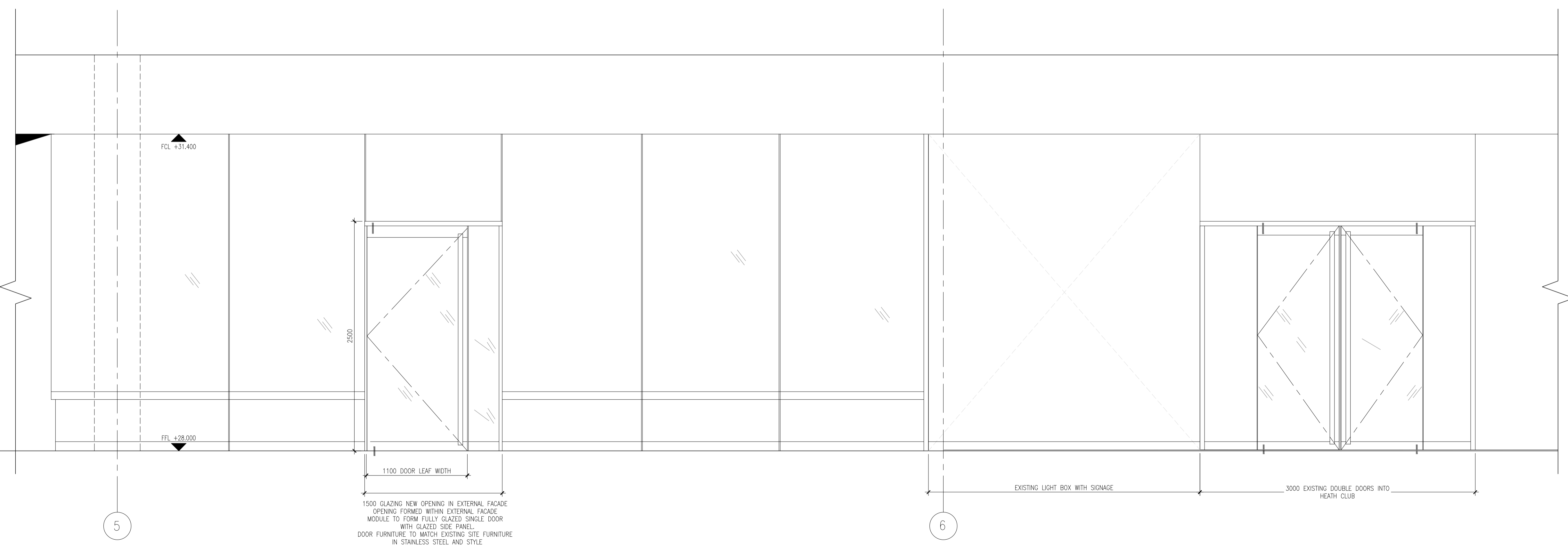
1 ELEVATION: NEW DOORSET INTO EXISTING CURTAIN WALL SCALE 1:25
