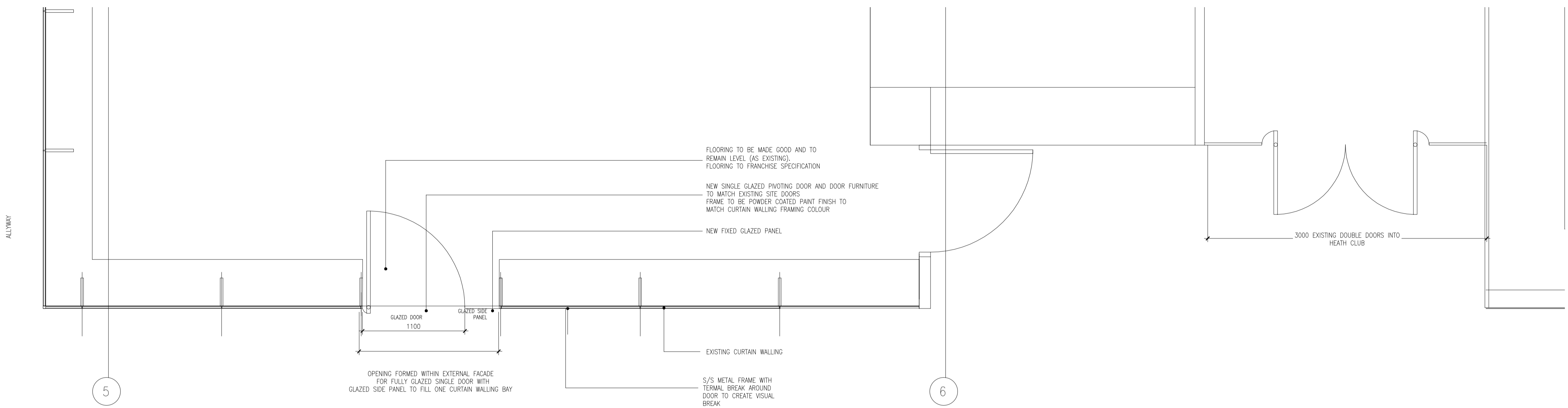
2 PLAN: NEW DOORSET INTO EXISTING CURTAIN WALL SCALE 1:25
