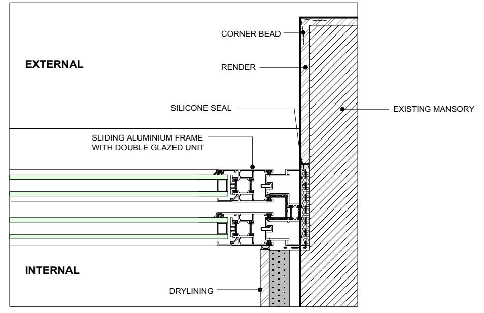
3 DETAIL JAMB. CONSERVATORY 1:5
