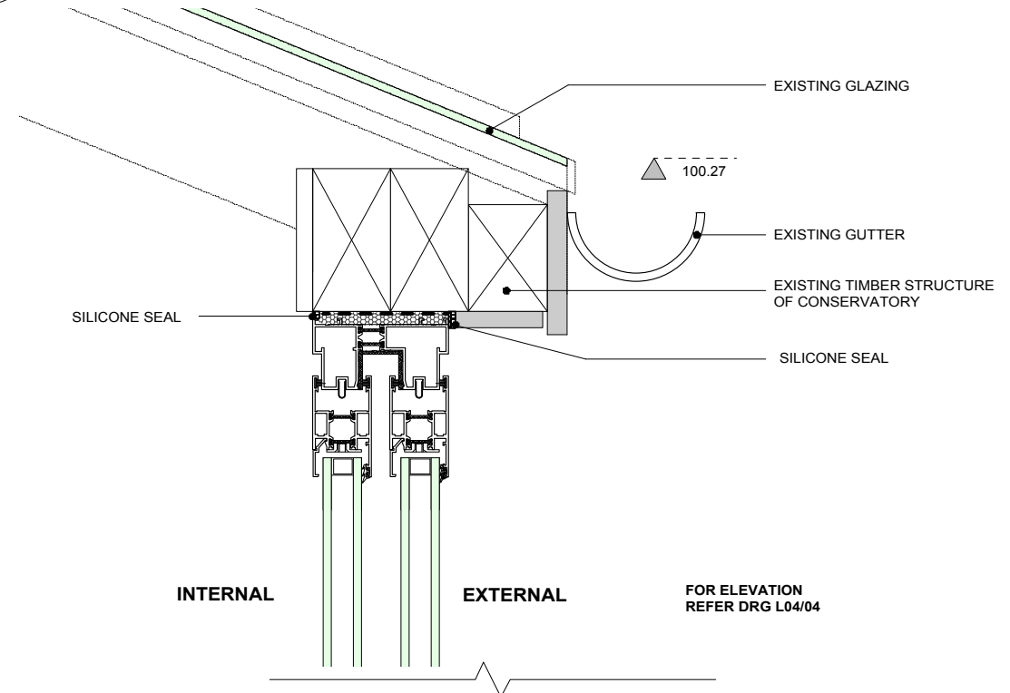
1 DETAIL HEAD. CONSERVATORY WINDOW 1:5
