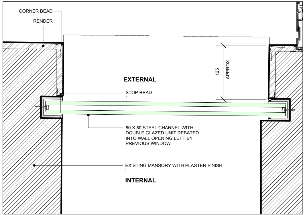
3 DETAIL JAMB, KITCHEN 1:5
