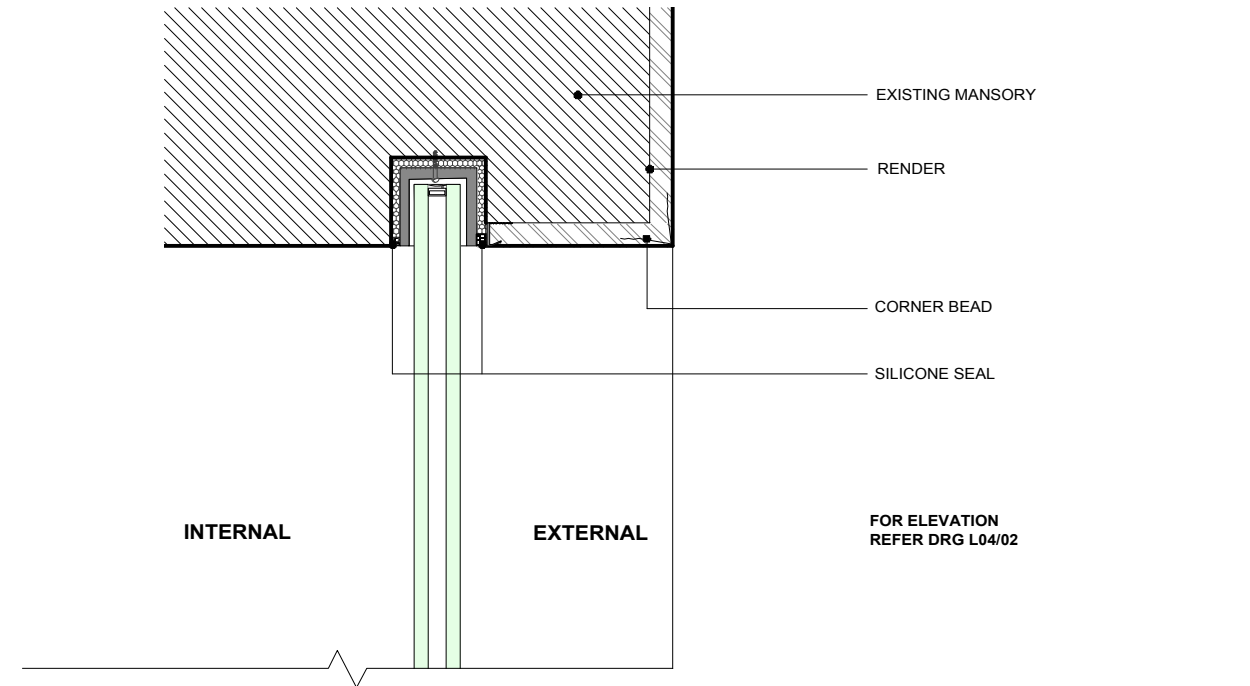
3 DETAIL JAMB, KITCHEN 1:5
