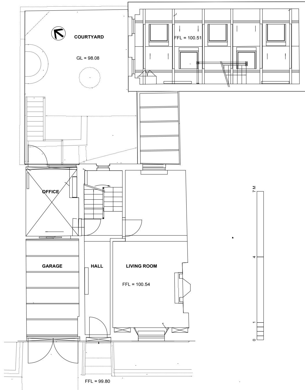
1 Ground Plan: (Existing as Proposed) 1:50@A1 / 1:100@A3
