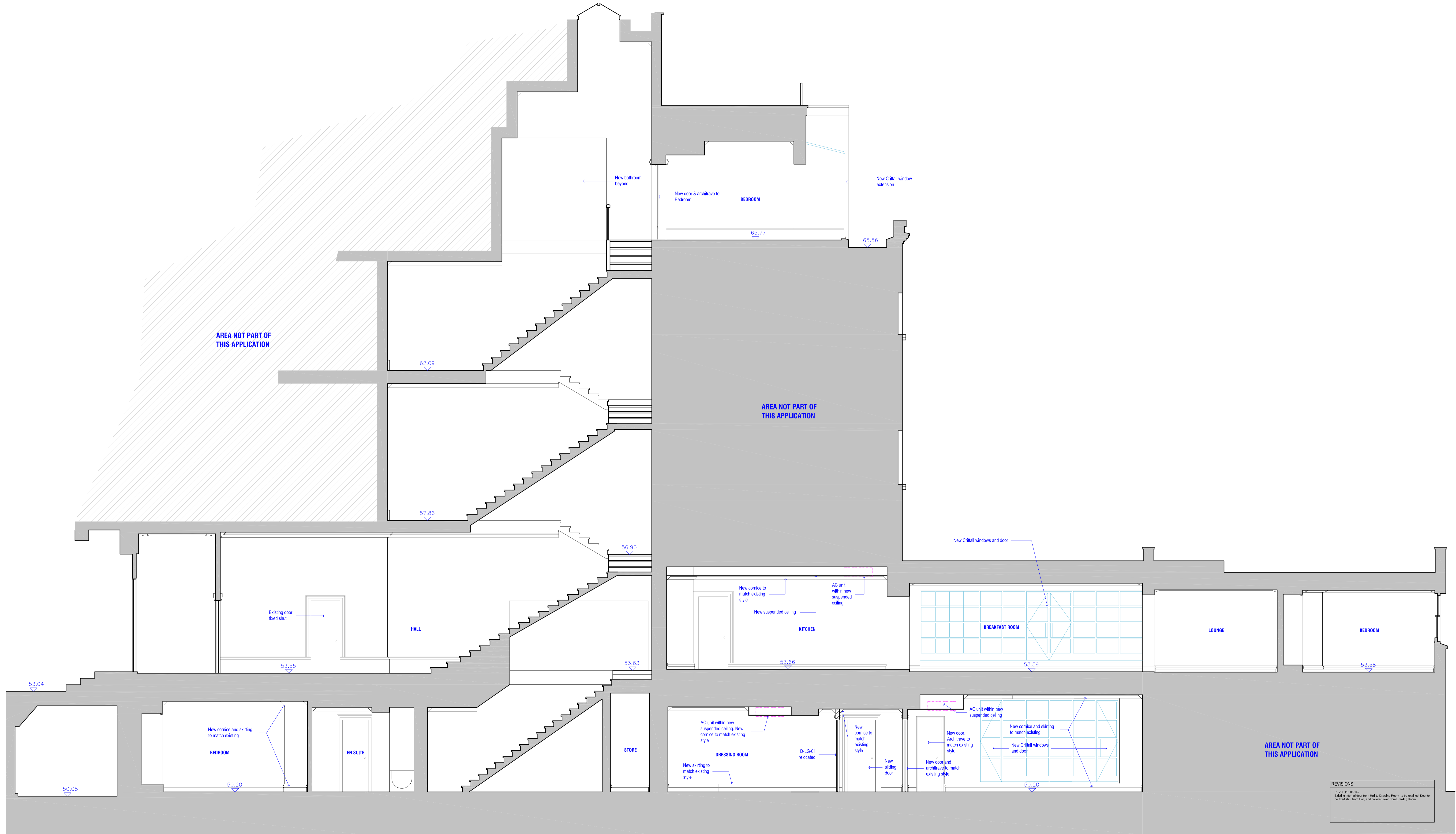
[01] PROPOSED SECTION B-B
