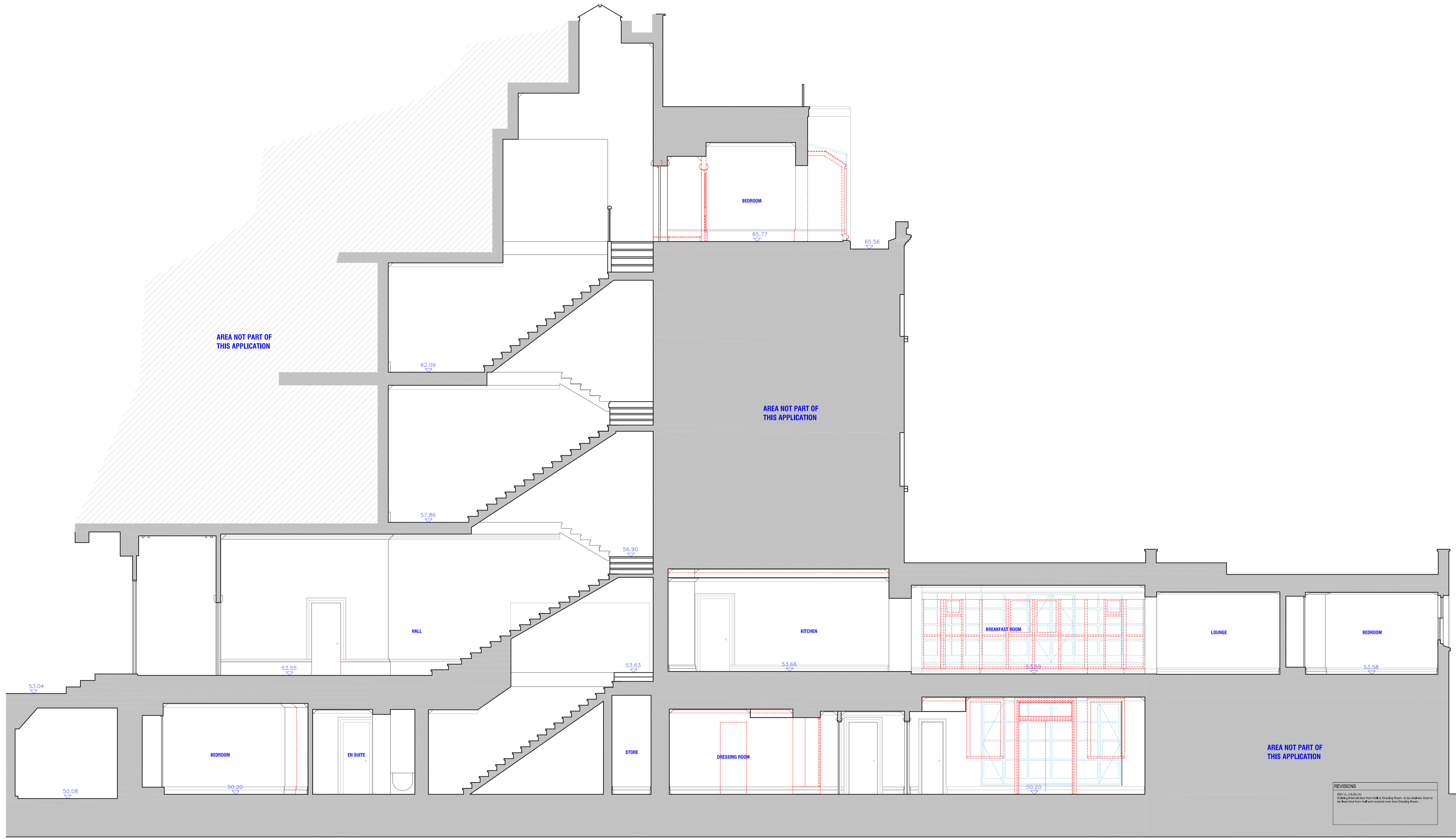
[01] DEMOLITION - SECTION B-B
