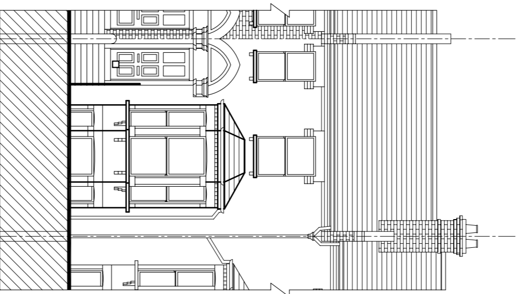
FRONT ELEVATION AS EXISTING
