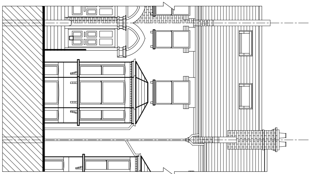
FRONT ELEVATION AS PROPOSED
